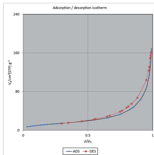
Fig. 3 N 2 adsorption-desorption isotherms of [Fe 3 O 4 @PAM-Schiff base-Mn][ClO 4 ] MNPs.
