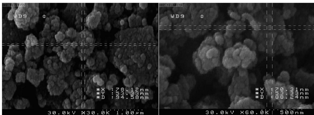
Fig. 7 SEM images of [\text{Fe}_3\text{O}_4@PAM\text{-Schiff base-Mn}][\text{ClO}_4] MNPs.
