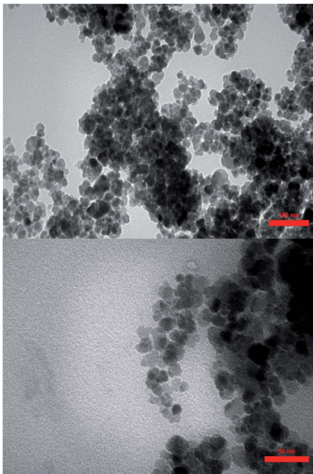
Fig. 8 TEM images of [\text{Fe}_3\text{O}_4@PAM\text{-Schiff base-Mn}][\text{ClO}_4] MNPs.
