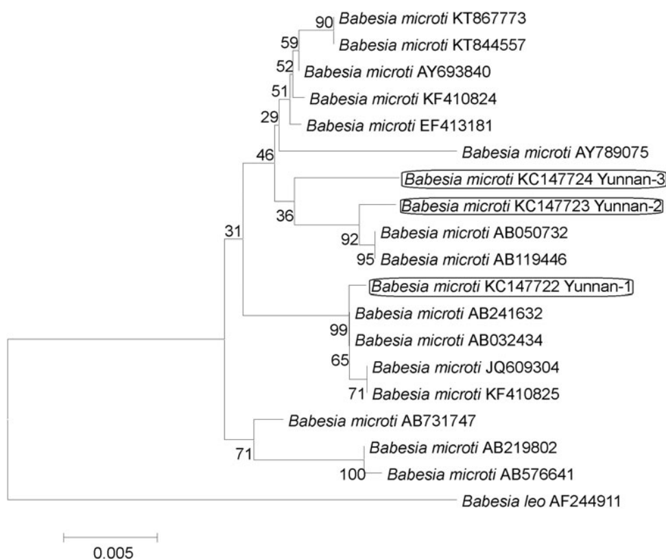
Fig. 2. Neighbor-joining tree of Babesia microti inferred from the 1078 bp sequence of 18S rRNA gene using the Neighbor-joining algorithm method with the Kimura two-parameter model. The number on each branch denotes the percent occurrence in 1000 bootstrap replicates. Three genetically different B. microti variants, Yunnan-1, Yunnan-2 and Yunnan-3, were detected. Yunnan-1, Yunnan-2 and Yunnan-3 were associated with Rattus (11/49, 22.5%), Apodemus (10/13, 76.9%) and Crocidura (5/10, 50.0%) species, respectively.
