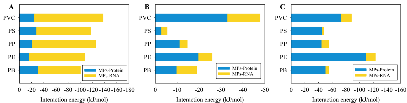
Fig. 1. Interaction energies of five types of MPs with the SARS-CoV-2 RNA fragment and the nucleocapsid protein (A), the SARS-CoV-1 RNA fragment and the nucleocapsid protein (B), as well as the HBV RNA fragment and the nucleocapsid protein (C), as obtained by geometry optimization.
