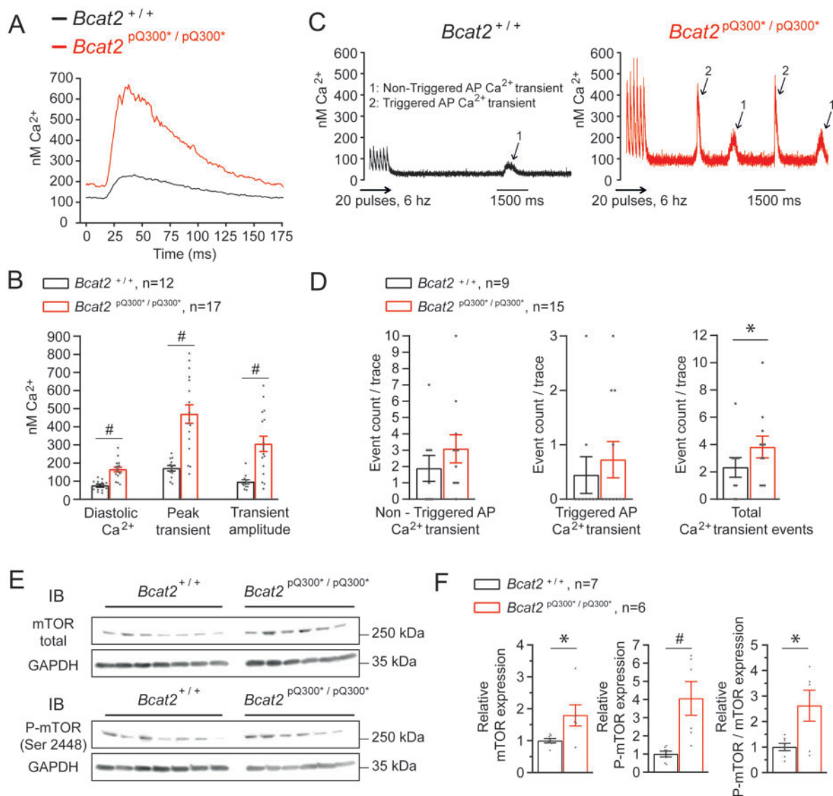
Figure 5 Abnormal intracellular calcium and myocardial mTOR upregulation in Bcat2^{p.Q300^*/p.Q300^*} mice. (A) Typical intracellular calcium transient recording performed at a pacing frequency of 6 Hz and (B) average values for diastolic Ca^{2+} , peak transient and transient amplitude of LV cardiomyocytes from Bcat2^{+/+} ( n = 12 cardiomyocytes from 5 independent cardiomyocyte dissociations) and Bcat2^{p.Q300^*/p.Q300^*} ( n = 17 cardiomyocytes from 4 independent cardiomyocyte dissociations) mice aged 4-5 weeks. (C) Typical example of calcium after-transients in isolated cardiomyocytes from Bcat2^{+/+} and Bcat2^{p.Q300^*/p.Q300^*} cardiomyocytes following a fast pacing protocol using field stimulation and (D) quantification of non-triggered action potential (AP) Ca^{2+} transient, triggered AP Ca^{2+} transient and total Ca^{2+} transient events in Bcat2^{+/+} ( n = 9 cardiomyocytes from 3 mice) and Bcat2^{p.Q300^*/p.Q300^*} mice ( n = 15 cardiomyocytes from 4 mice). (E) Representative immunoblots of total mTOR, phosphorylated mTOR (P-mTOR) at ser2448 and GAPDH from heart lysates (apex) from Bcat2^{+/+} and Bcat2^{p.Q300^*/p.Q300^*} mice. (F) Average total mTOR and phosphorylated P-mTOR expression normalized to GAPDH, and ratio of normalized P-mTOR on normalized total mTOR from Bcat2^{+/+} ( n = 7 ) and Bcat2^{p.Q300^*/p.Q300^*} ( n = 6 ) mouse heart lysates. * P < 0.05 ; # P \leq 0.001 (with Student's t -test or Mann-Whitney Rank sum test).
