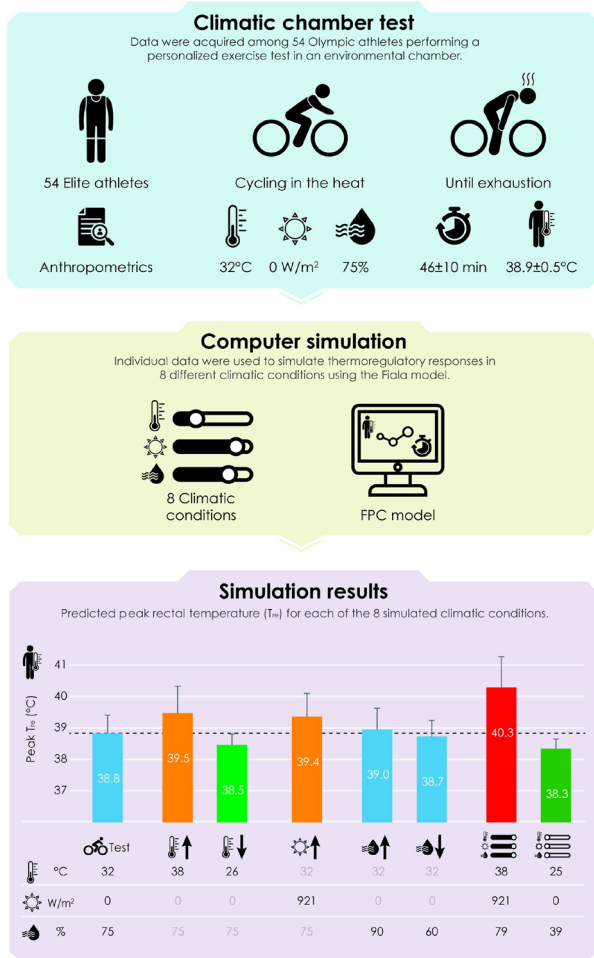
Figure 2 Outcomes of the computer simulation of eight distinct climatic conditions on peak rectal temperature ( T_{re} ) of elite athletes exercising in the heat. An isolated increase in air temperature and solar radiation led to a higher peak T_{re} , but the impact of the worst-case scenario on peak T_{re} was greater than the sum of its parts. FPC, Fiala-thermal-Physiology-and-Comfort.
