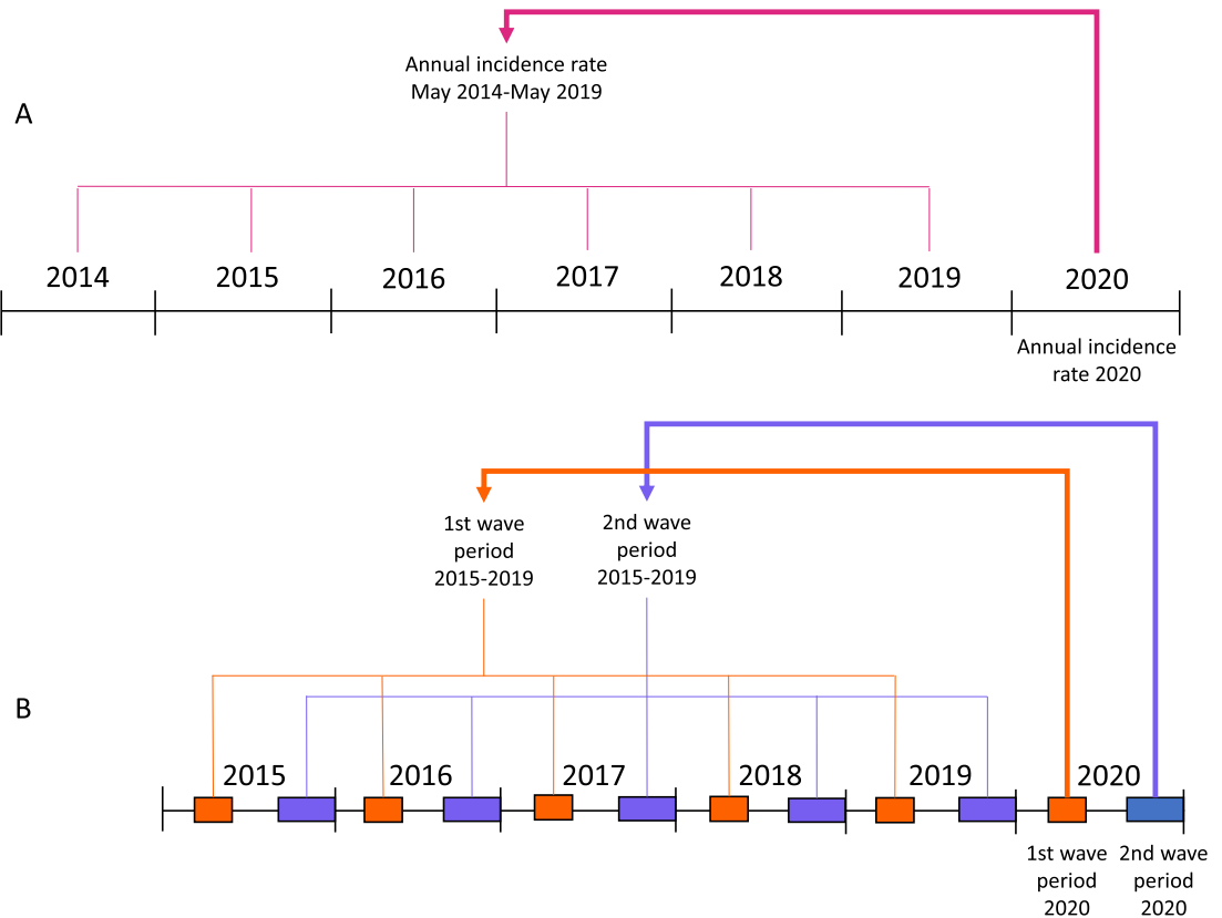
Figure 1. Overview of the performed analyses in this study. A: Comparison of the annual incidence rates of 2020 with the previous five surveillance years (year-level). B: Comparison of the percentages of CDI patients with certain characteristics in the wave periods in 2020 with that of CDI patients in the same calendar periods (wave periods) in 2015 through 2019 (patient-level).
