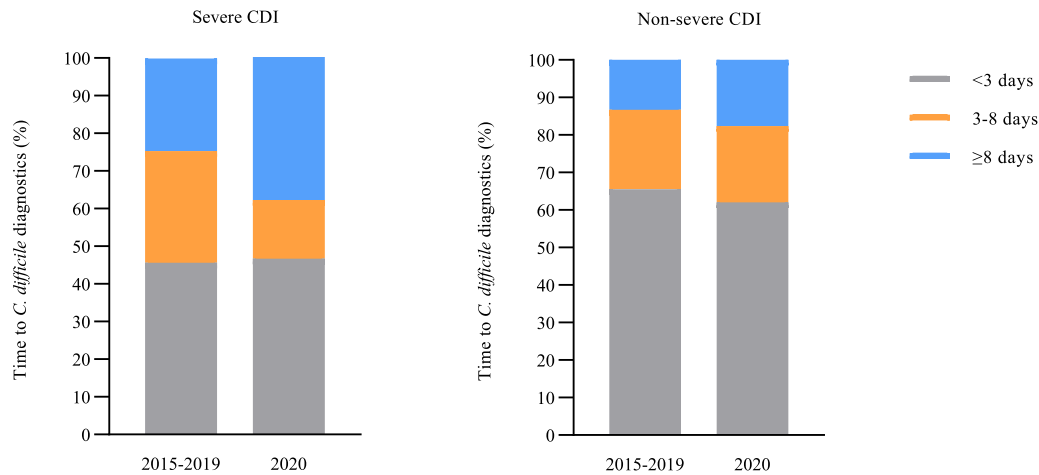
Figure 2. Time to C. difficile diagnostics in the second wave in 2020 compared to the same period in 2015 through 2019 for severe CDI and non-severe CDI patients.
