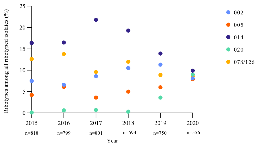
Figure 3. Percentage of five most common ribotypes of 2020 in time from 2015 through 2020.
