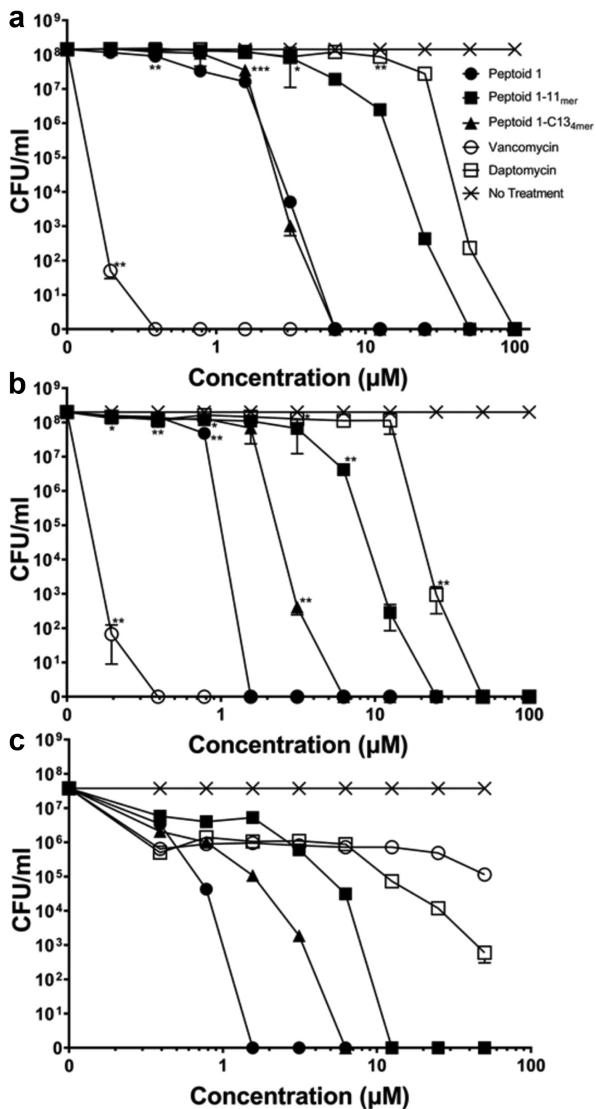
FIG 2 CFU/ for drug-resistant/drug-sensitive strains of S. aureus (a) Xen36, (b) MRSA 252, and (c) Xen 29 with Peptoid 1, Peptoid 1-C13 4mer , Peptoid 1-11 mer , and traditionally used antibiotics vancomycin and daptomycin at various concentrations on LB plates after 24 h. (a) For Xen36, vancomycin was significantly different from the no treatment control at 0.19 \mu M and above, while Peptoid 1 was significant starting at 0.78 \mu M and above. Peptoid 1-C13 4mer showed significance starting at a concentration of 3.125 \mu M. Peptoid 1-11 mer showed significance at 0.19 \mu M but didn't show significance again until 0.78 \mu M.
