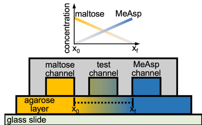
FIGURE 2 Side view of the three-channel microfluidic device used to expose cells to constant chemoattractant gradients. The channels, fabricated in solute-impermeable polydimethylsiloxane, were 20-mm long, 100- \mu m deep, and 600- \mu m wide, with 400- \mu m spacing between each channel. The agarose layer was 0.5-mm thick. Motility medium with a constant maltose concentration was flowed through the left outer channel, and motility medium with a constant MeAsp concentration was flowed through the right outer channel. For the opposing-gradient experiments, both the maltose and MeAsp concentrations were nonzero; for the single-gradient experiments, one of the two outer channels contained only motility medium. The chemoattractants diffused through the agarose layer and up into the test channel, creating two steady linear concentration profiles in opposite directions. This figure was adapted from (46). To see this figure in color, go online.
