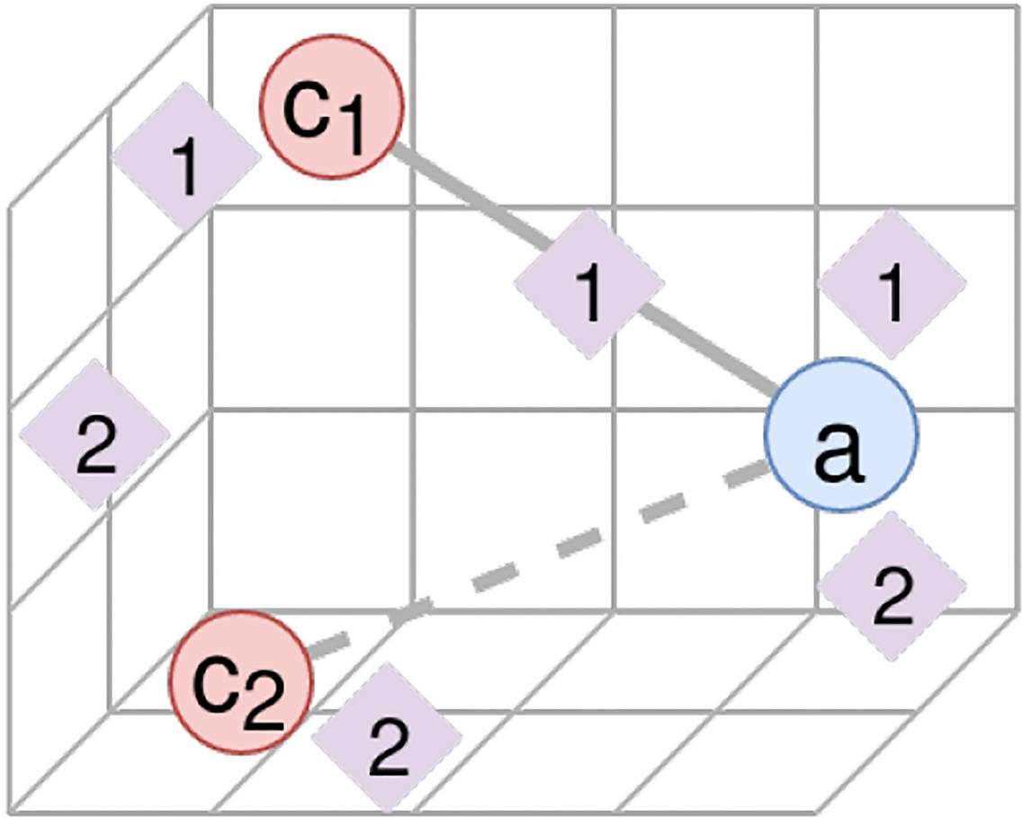
Fig. 2. The above depicts two queries, a-c_1 and a-c_2 , where a-c_1 is a published connection and a-c_2 is a noise connection. We see topics for each query represented as diamonds via CENTR(T_i) . Although both queries lead to topics which are similar to a , c_1 , or c_2 , we find that the presence of some topic which is similar to both objects of interest may indicate the published connection.
