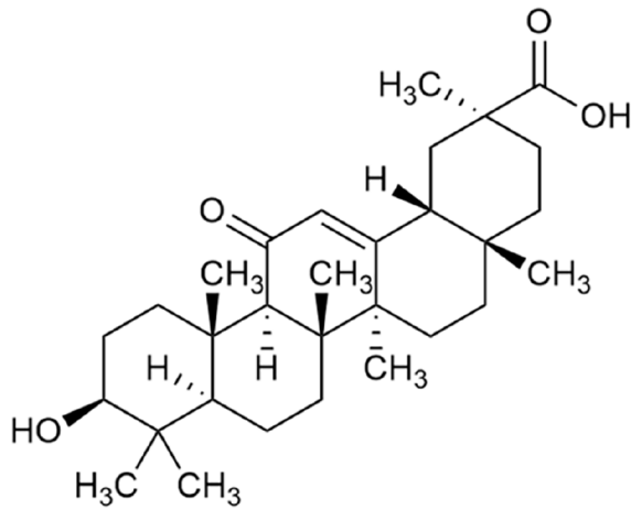
Figure 1 Structure of 18 \beta -glycyrrhetic acid. The molecular formula for 18 \beta -glycyrrhetic acid is C 30 H 46 O 4 , and the molecular weight is 470.68.
