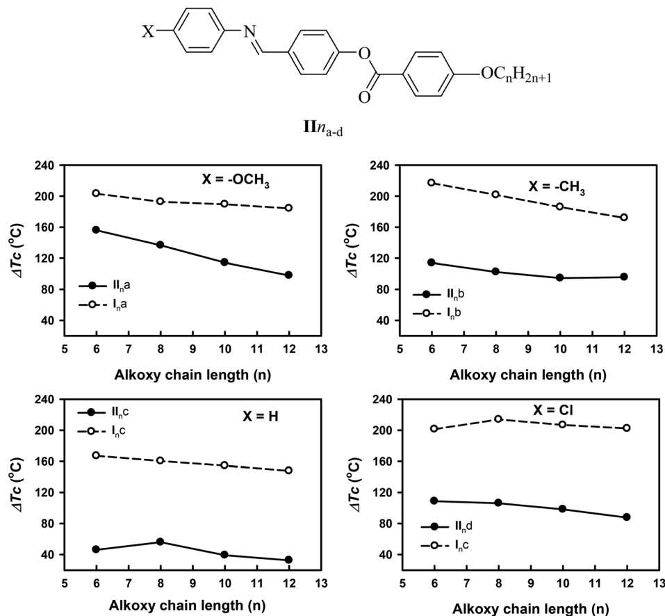
Fig. 5 Comparison of \Delta T_c of the 4-ring ( \text{I}_{n-a-d} ) and 3-ring ( \text{II}_{n-a-d} ) analogues.
