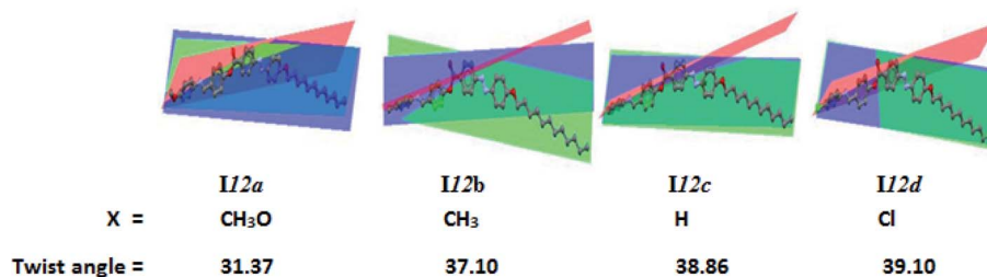
Fig. 6 Calculated geometrical structures of compounds \text{I12}_{a-d} .
