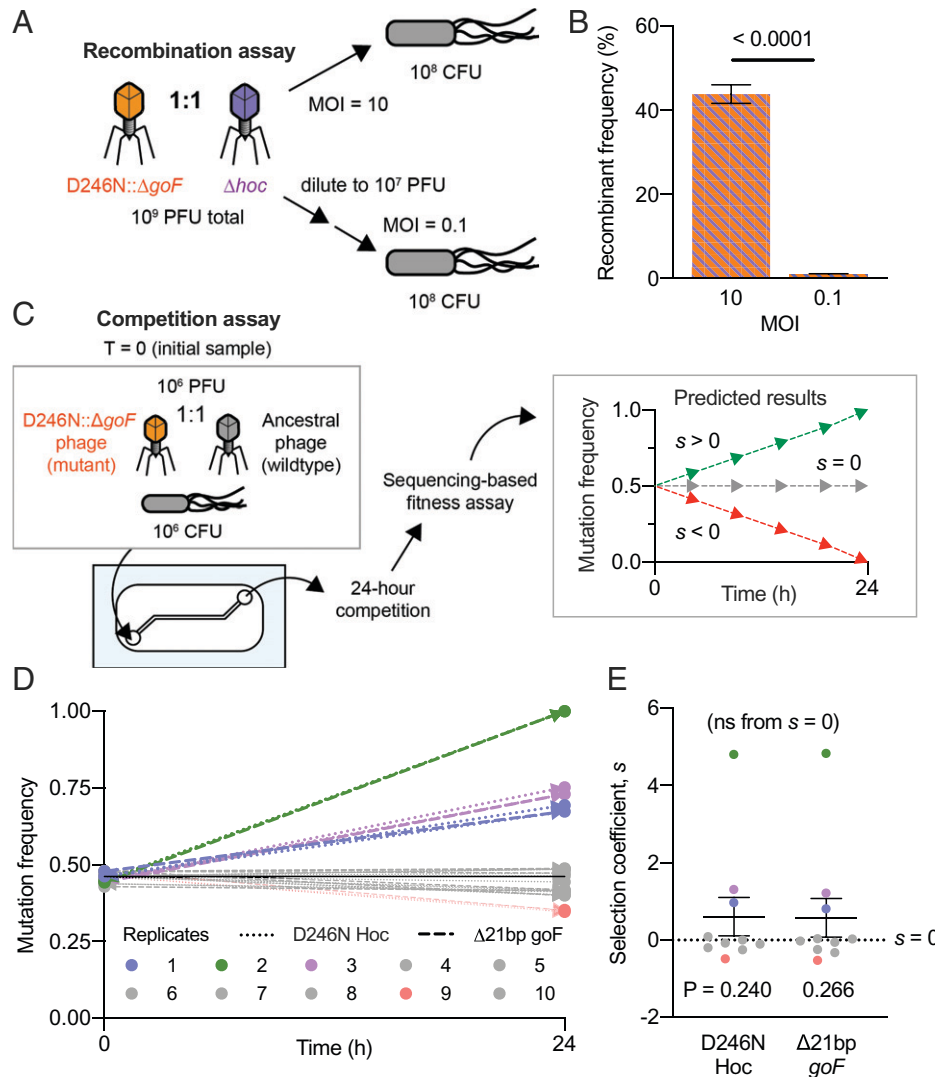
Fig. 3. Mucus layer supports phage recombination and selection of beneficial mutants. (A) A gut-on-a-chip-evolved D246N:: \Delta goF phage mutant was mixed at a 1:1 ratio with a laboratory-derived \Delta hoc mutant. Naive E. coli were infected with the 1:1 phage mixture at MOIs 10 and 0.1 following a one-step growth protocol to ensure that only a single round of viral replication could occur. (B) Percentage frequency of phage recombinants from PCR screening for \Delta 21bp goF - \Delta hoc or wild type-reconstituted recombinants. Forty-nine phage isolates ( n = 49 ) were screened per experimental replicate. There were two experimental replicates ( n = 2 ) leading to a total of 98 phage isolates ( n = 98 ) screened per experimental condition (MOI 10 or 0.1) (SI Appendix, Fig. S5). (C) Competition experiment between the D246N:: \Delta goF phage mutant with ancestral phage T4 in the gut-on-a-chip. A gut-on-a-chip seeded with naive E. coli was inoculated with equal proportions of the respective phage genotypes. Chip effluents were collected for 1 h at 24 h of competition and the samples were subjected to whole-genome sequencing to track D246N Hoc and \Delta 21bp goF mutations after 24 h of competition. Estimated selection coefficients could be positive ( s > 0 ), neutral ( s = 0 ), or negative ( s < 0 ). (D) D246N Hoc and \Delta 21bp goF mutational frequencies measured from 10 independent gut-on-a-chip replicates ( n = 10 ) between the initial inoculum, namely T = 0 and 24 h. (E) Plot of the estimated mean selection coefficient for D246N Hoc and \Delta 21bp goF mutations across 10 experimental replicates ( n = 10 ). The black solid line in D represents the initial ( T = 0 ) average frequency of D246N Hoc mutation at 45.8% and \Delta 21bp goF mutation at 46.7%, across 10 experimental replicates ( n = 10 ). Error bars in B and the line with error bars in E represent mean \pm SEM across experimental replicates (B: n = 2 , i.e., two experimental replicates, n = 98 screened per experimental replicate; E: n = 10 , i.e., ten experimental replicates). P values in B were derived from an unpaired two-tailed t test between treatment conditions (MOI 10 and 0.1). P values in E were derived from an unpaired two-tailed t test between coefficients of D246N Hoc and \Delta 21bp goF mutations against s = 0 (no significance; ns), respectively.
