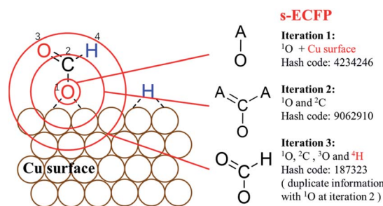
Fig. 2 Procedure to generate identifiers for molecules on surfaces using Surface-sensitive atom-centered Extended-Connectivity FingerPrint (s-ECFP). The iterative procedure for generating s-ECFP is illustrated using the adsorbed O end ( ^1\text{O} ) of HCOO as the example. Each iteration creates an identifier for the substructure in a circle around the central atom. The identifier at iteration 1 only represents the information of the ^1\text{O} atom, its attached bonds and the surface in bonding. By enlarging the circles, the next iterations include more and more information associated with the substructure centering on the ^1\text{O} . Duplicate identifiers will be removed, for example, the substructure of ^1\text{O} at the iteration 3 is the same as the one of atom ^2\text{C} at the iteration 2. The explanatory text in red indicates the added features for s-ECFP compared to the ECFP.
