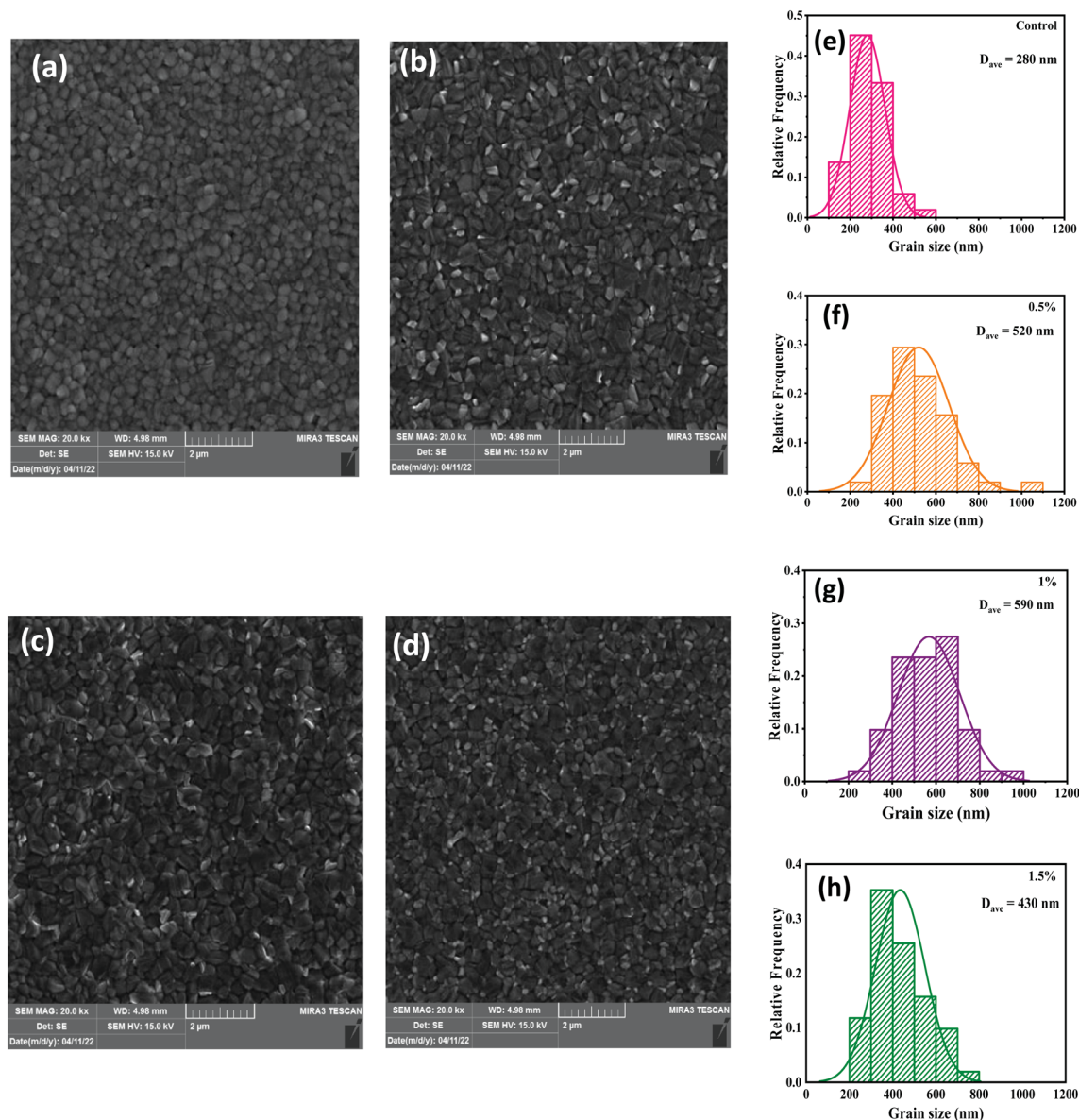
Fig. 1 The top-view FESEM visualization of perovskite layers with (a) 0%, (b) 0.5%, (c) 1%, and (d) 1.5% of \text{CdCl}_2 in perovskite precursors. Substrate for all layers was FTO/c-TiO 2 /mp-TiO 2 . (e–h) Particle size distributions of perovskite films evaluated by ImageJ software.
