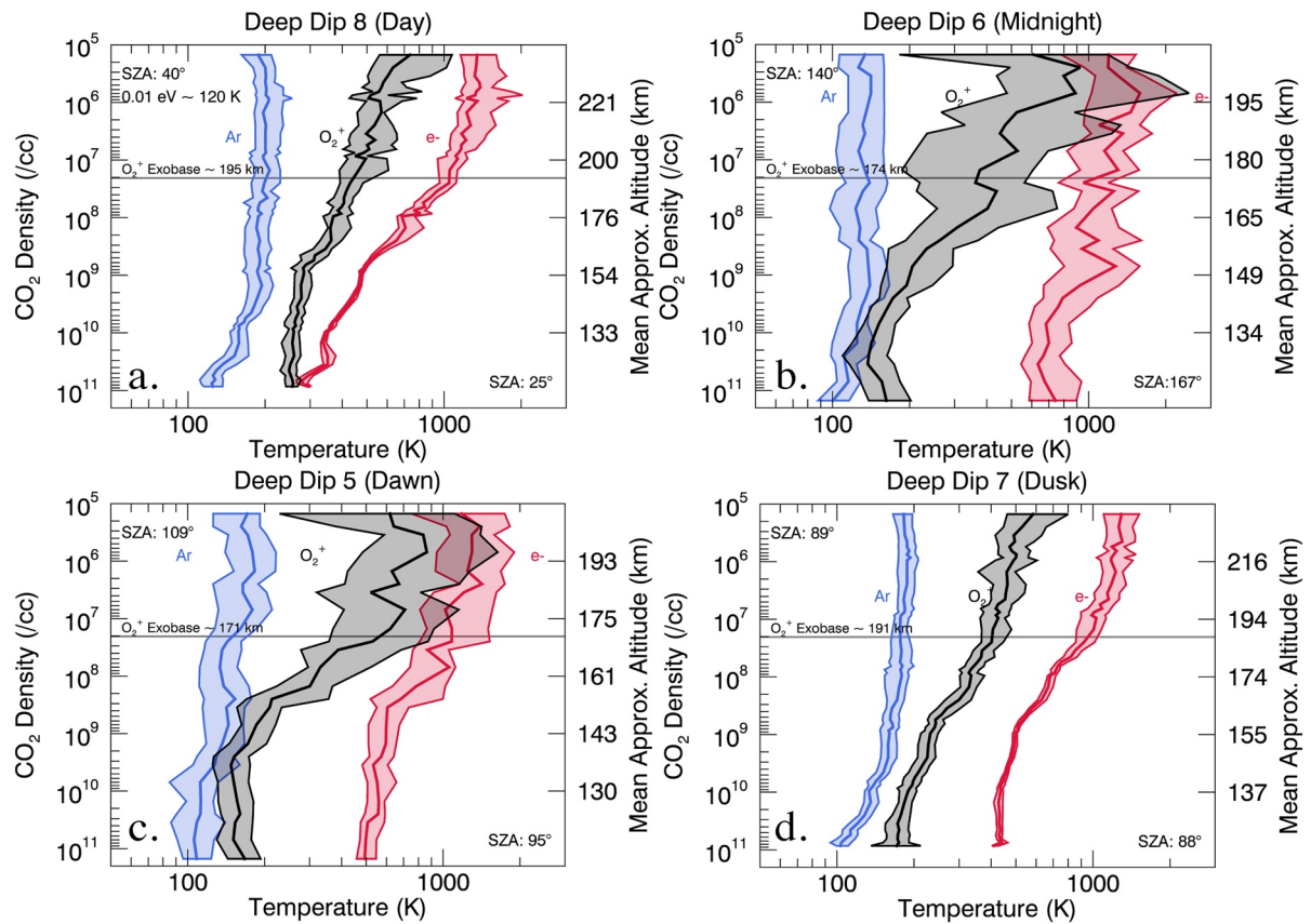
Figure 7. Median temperature profiles as a function of \text{CO}_2 density for \text{O}_2^+ , Ar, and electrons collected during (a) Deep Dip (DD) 8 at 14:00 local time, (b) DD 6 at 01:00, (c) DD 5 at 05:00, and (d) DD 7 at 20:00. \text{O}_2^+ temperatures from STATIC are shown in black, neutral Ar temperatures measured by Mars Atmosphere and Volatile EvolutionN (MAVEN) NGIMS are shown in blue, and electron temperatures from MAVEN LPW are shown in red. Shaded regions represent upper and lower quartiles. Solar zenith angles at the top and bottom of the profiles, which vary by 16^\circ at most, are indicated on the plots. Exobase altitudes indicate where the ion scale height exceeds the mean free path between ion-neutral collisions.
