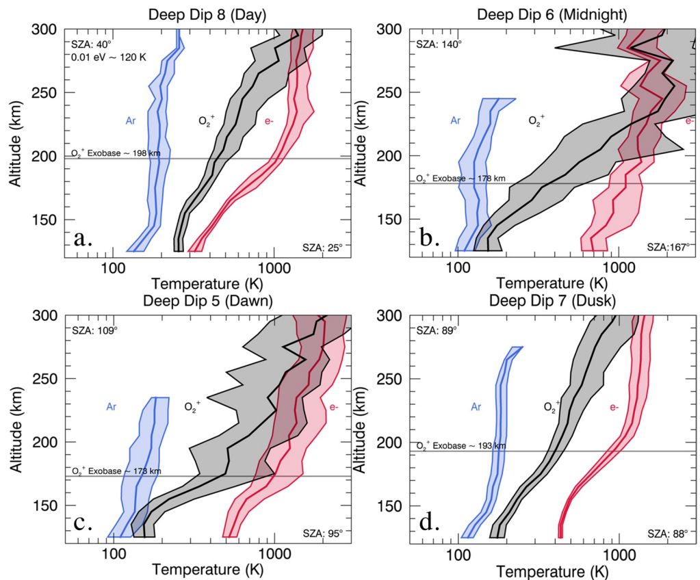
Figure 6. Median temperature profiles as a function of altitude for \text{O}_2^+ , Ar, and electrons collected during (a) Deep Dip (DD) 8 at 14:00 local time, (b) DD 6 at 01:00, (c) DD 5 at 05:00, and (d) DD 7 at 20:00. \text{O}_2^+ temperatures from STATIC are shown in black, neutral Ar temperatures measured by Mars Atmosphere and Volatile EvolutionN (MAVEN) NGIMS are shown in blue, and electron temperatures from MAVEN LPW are shown in red. Shaded regions represent upper and lower quartiles. Solar zenith angles at the top and bottom of the profiles, which vary by 16^\circ at most, are indicated on the plots. Exobase altitudes indicate where the ion scale height exceeds the mean free path between ion-neutral collisions.
