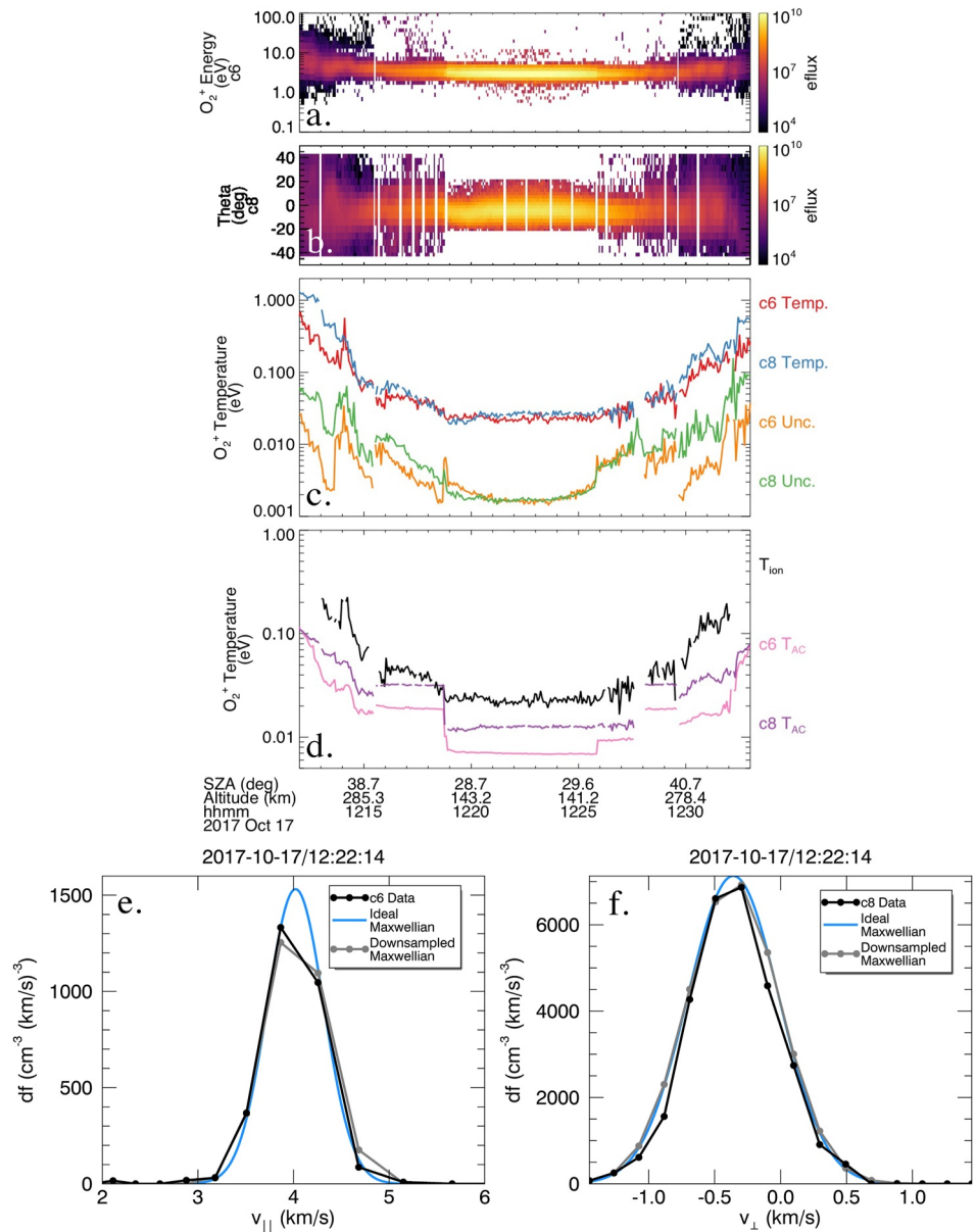
Figure 2. Panel (a) c6 energy spectrogram for O 2 + during one periapsis pass. Energy flux has units of eV/cm 2 /s/steradian/eV. Panel (b) c8 deflector angle distribution. Panel (c) Measured O 2 + energy (angular) beamwidth temperatures in red (blue), and associated statistical uncertainties in orange (green). Panel (d) Final O 2 + temperature in black and analyzer corrections for the energy and angular beamwidths in pink and purple. Discontinuities in T AC correspond to changes in mode and attenuator state, which impact instrument resolution. Solar zenith angle and altitude are indicated at the bottom of the plot. Panel (e) A c6 distribution function, not corrected for spacecraft motion. The blue line is not fitted to the data, but represents an ideal Maxwell-Boltzmann distribution with the same temperature and bulk velocity as the measured distribution. The peak of the measured distribution function is used as a scaling factor. The ideal Maxwellian is downsampled by averaging over each STATIC energy bin to produce the gray points. Panel (f) A c8 distribution function. The blue and gray Maxwellians are produced using the same process as panel (e). The magnitudes of the distribution functions differ due to assumptions made about the angular coverage of the distribution for c6 data.
