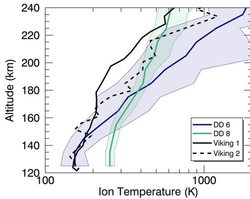
Figure 4. Median O_2^+ temperature profiles measured by STATIC during Deep Dips 6 and 8 compared to the Viking RPA ion temperatures. Shaded regions indicate upper and lower quartiles for each 10-km altitude bin.
