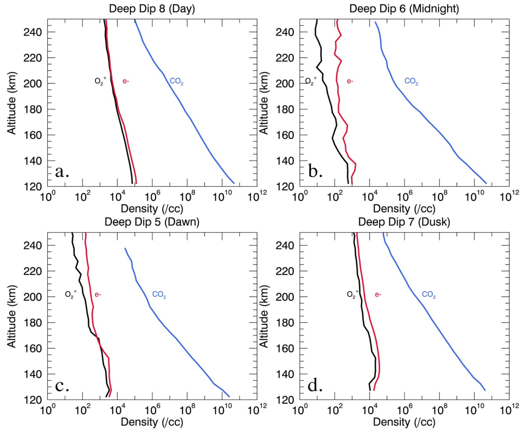
Figure 8. Median density profiles as a function of altitude for O_2^+ , CO_2 , and electrons collected during (a) Deep Dip (DD) 8 at 14:00 local time, (b) DD 6 at 01:00, (c) DD 5 at 05:00, and (d) DD 7 at 20:00. O_2^+ densities from STATIC are shown in black, neutral CO_2 densities measured by Mars Atmosphere and Volatile EvolutionN (MAVEN) NGIMS are shown in blue, and electron densities from MAVEN LPW are shown in red. Differences in O_2^+ and electron densities are partly due to the presence of additional ion species. Larger discrepancies may occur at high altitudes because uncertainties in electron density increase as the density decreases (Fowler et al., 2015). These differences do not significantly affect model output.
