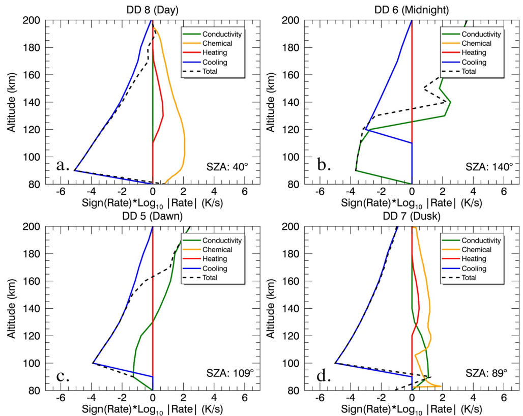
Figure 9. Heating and cooling rates for O_2^+ during DDs 5–8 assuming a single solar zenith angle as indicated on each plot. The log of each rate in K/s is plotted on the x -axis, where negative rates indicate cooling and positive rates indicate heating. Rates below 1 K/s, which would result in a negative log, were excluded from the data set. The thermal conductivity term accounts for the effects of temperature gradients, the heating rate represents the energy gained through Coulomb collisions with electrons, and the cooling rate represents the energy lost through collisions with neutrals. The conductivity, heating, and cooling terms are calculated using the Matta et al. (2014) ionosphere model. The chemical heating term represents energy deposited by atmospheric chemistry and is calculated as described in the text.
