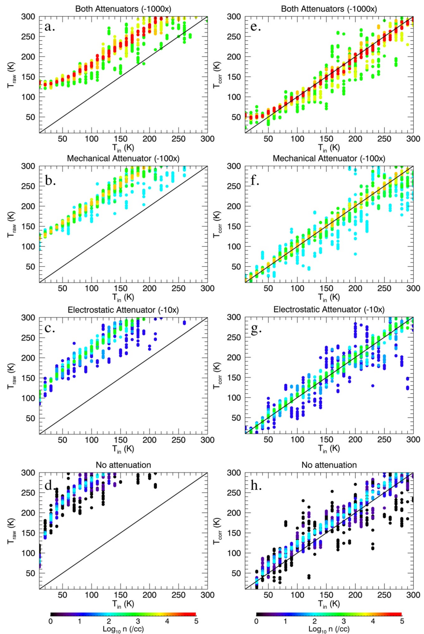
Figure 3. O_2^+ energy beamwidth temperatures, (a–d) raw and (e–h) corrected for analyzer response, as a function of the temperature T_{in} of a simulated Maxwellian distribution measured with a simulated STATIC. Color indicates the density of the simulated distribution function. Each row of figures represents a different attenuator state; the number in parentheses indicates the factor by which the ram flux is reduced. The effects of ion suppression and scattering are not included in the simulation. Ion suppression does not affect the temperature measurement; T_{scatter} is zero during the passes analyzed in this work.
