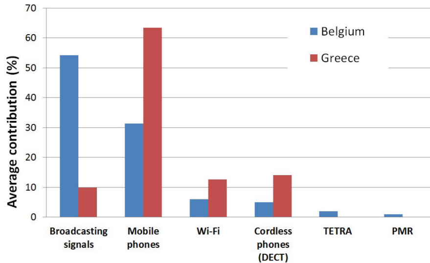
Figure 1 Average contribution (%) of various RF signals measured as electric field strength (V/m) in Belgian and Greek schools (7)
