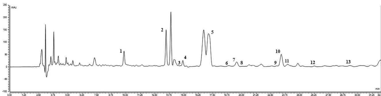
FIGURE 1 Chromatogram of maca sample: (1) unknown macamide; (2) linolenic acid; (4) n -benzyl-(9Z, 12Z, 15Z)-octadecatrienamide; (5) linoleic acid; (7) n -benzyl-(9Z, 12Z)-octadecadienamide; (8) n -benzylpentadecanamide; (9) n -(3-methoxybenzyl)-hexadecanamide; (10) n -benzylhexadecanamide; (11) n -benzyl-(9Z)-octadecanamide; (12) n -benzylheptadecanamide; (13) n -benzyloctadecanamide. (3) and (6) are probably methoxy-derivatives of 4 and 7, respectively
