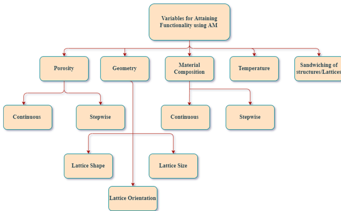
Fig. 3. Variables for FGAM
