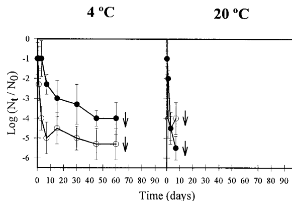
FIG. 1. Reduction of the infectivity of human AsV, expressed as log 10 (RT-PCR t /RT-PCR 0 ), during 90 days dried on china at 4 and 20°C at a relative humidity of 90% \pm 5% (open circles, PBS suspension; solid circles, 20% fecal suspension). Error bars indicate standard deviations. Arrows indicate the limit of detection.
