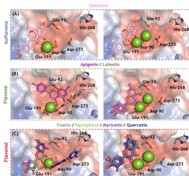
Figure 4. The electrostatic potential map ( -68.065 and +68.065 a.u., in red and blue, respectively) of the best docking poses for the flavonoids (A) isoflavone, (B) flavones, and (C) flavonols in the SARS-CoV-2 nsp14 ExoN active site in the presence of one and two Mg(II) ions (left and right, respectively). The catalytic amino acid residues, genistein, apigenin, luteolin, fisetin, kaempferol, myricetin, and quercetin are in stick representation in cyan, violet, pink, brown, gray, light green, purple, and marine, respectively. Mg(II) and Zn(II) ions are represented as green and indigo blue spheres, respectively. Hydrogen, oxygen, and nitrogen are shown in white, red, and dark blue, respectively.
