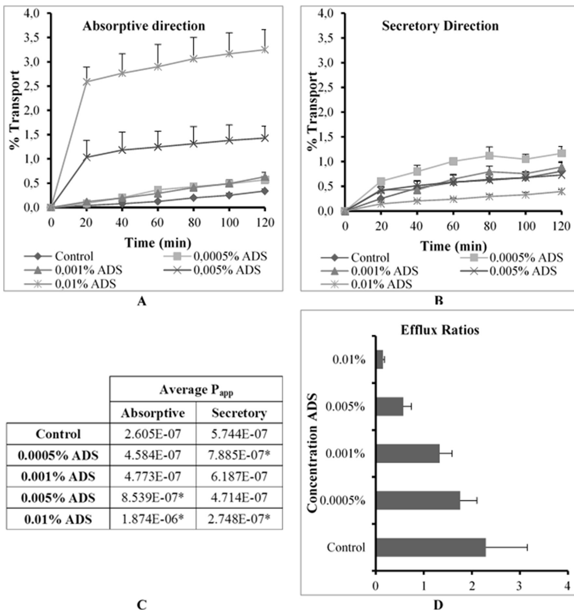
Fig. 2 – Graphical presentation of the percentage transport of Rhodamine 123 in the (A) absorptive and (B) secretory directions (C) apparent permeability coefficient (P app ) values for bi-directional transport and (D) the efflux ratio (ER) values in the presence of Ac-di-sol® (ADS) at four concentrations across excised pig intestinal tissues (* indicates statistically significant differences from the control, p ≤ 0.05).
