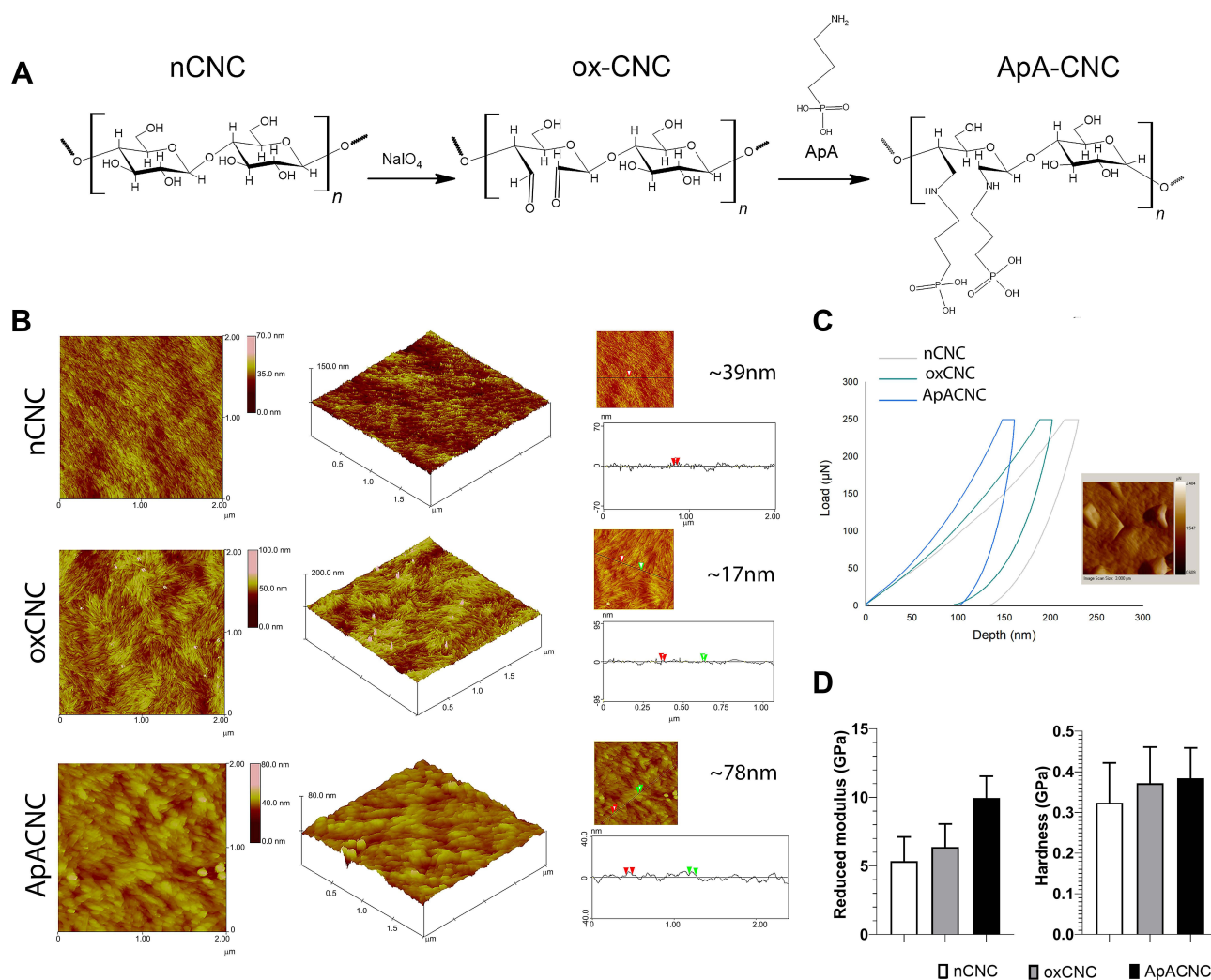
Figure 1 Characterization of native, oxidized and ApA-modified CNCs. (A) Chemical structures of CNCs used in the study. (B) AFM images of top-view analysis (scan size of 2 \times 2 \mu\text{m} ) (left), surface area plot analysis (middle), and cross-section analysis with indicated nanocrystal thickness measurements (right, marked by red or green triangles) are shown. (C) Nanoindentation analysis for native and modified CNCs, and scanning probe microscope (SPM) image showed the indents at ApA-CNCs (scan size of 3 \times 3 \mu\text{m} ). (D) Summarized data for reduced elasticity and hardness is shown as mean \pm SD of 9 randomly selected measurements on the same CNC preparation. Surface plot analysis.
