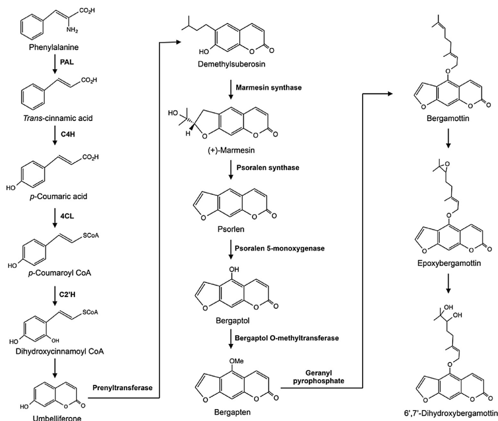
Figure 1 – Biosynthetic pathway of 6',7'-dihydroxybergamottin in citrus fruits. 4CL = 4-coumarate-CoA ligase; C2'H = cinnamoyl-CoA 2'hydroxylase; C4H = cinnamate 4-hydrolase; PAL, phenylalanine ammonia-lyase.
