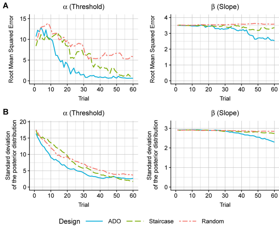
Fig. 6: Comparison of ADO, staircase, and random designs in the simulation of psychometric function estimation. Simulations were conducted using the logistic model with parameter values of threshold \alpha = 20 , slope \beta = 1.5 , guess rate \gamma = 0.5 , and lapse rate \delta = 0.04 . The three designed are compared with root mean squared errors (RMSE; Panel A) and standard deviations of the posterior distribution (Panel B). RMSE represents the discrepancy between true and estimated parameters in that the lower RMSE, the better estimation performance. Standard deviations of the posterior distribution indicate the certainty of a belief on the distribution for model parameters, i.e., the lower the standard deviations is, the higher certainty on the model parameters. Each curve represents an average across 1,000 independent simulation runs.
