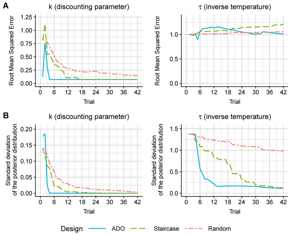
Fig. 7: Comparison of ADO, staircase, and random designs in the simulation of the delay discounting task. Simulations were conducted using the hyperbolic model with parameter values of k = 0.12 and \tau = 1.5 . The three designs are compared with root mean squared errors (RMSE; Panel A) and standard deviations of the posterior distribution (Panel B). Each curve represents an average across 1,000 independent simulation runs.
