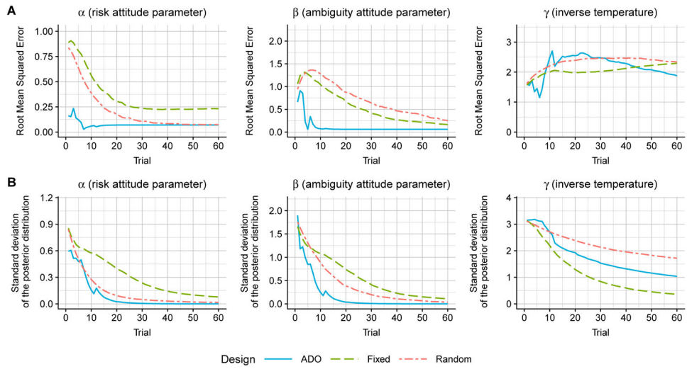
Fig. 9: Comparison of ADO, fixed, and random designs in the simulation of the choice under risk and ambiguity task. The fixed design was pre-determined according to Levy et al. (2010). Simulations were conducted using the linear model with parameter values of \alpha = 0.66 , \beta = 0.67 , and \gamma = 3.5 . Three designs are compared with root mean squared errors (RMSE; Panel A) and standard deviations of the posterior distribution (Panel B). Each curve represents an average across 1,000 independent simulation runs.
