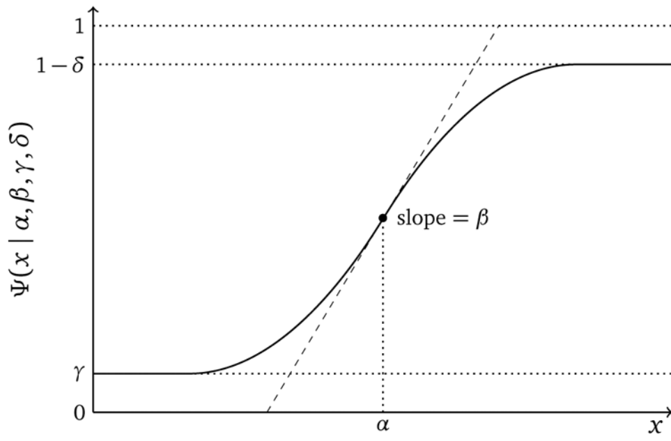
Fig. 5: The psychometric function and its parameters defined in Equation (4).
