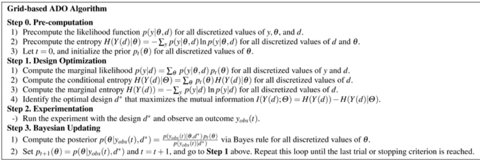
Fig. 2: Three steps of a grid-based ADO algorithm with an initial step for pre-computation.
