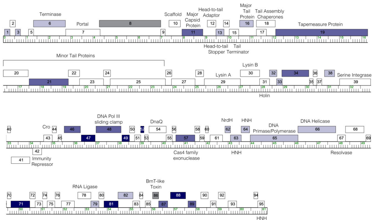
Fig. 1. The genome of phage Waterfoul. The Waterfoul genome is shown as a ruler with kbp markers and genes represented by boxes—those above the line are transcribed rightwards and those below are transcribed leftwards. Numbers inside the box correspond to gene numbers and predicted functions are indicated above each gene. Box shading corresponds to cytotoxicity scoring, with white boxes designating genes found to have no effect on M. smegmatis growth, gray boxes indicating genes for which transformants could not be recovered (+++; genes 8 and 86), and blue representing observed toxicity in our assay. The saturation of blue boxes corresponds to the severity of growth inhibition using the following scores: light blue (+; reduction in colony size; genes 1, 3, 6, 13, 16, 32, 33, 38, 62, 63, 64, 65, 66, 79, and 82), medium blue (++; 1–3 log reduction in viability; genes 11, 19, 21, 34, 46, 48, 57, 87, and 89), and dark blue (+++; >3-log reduction in viability; genes 47, 49, 52, 71, 81, and 88).
