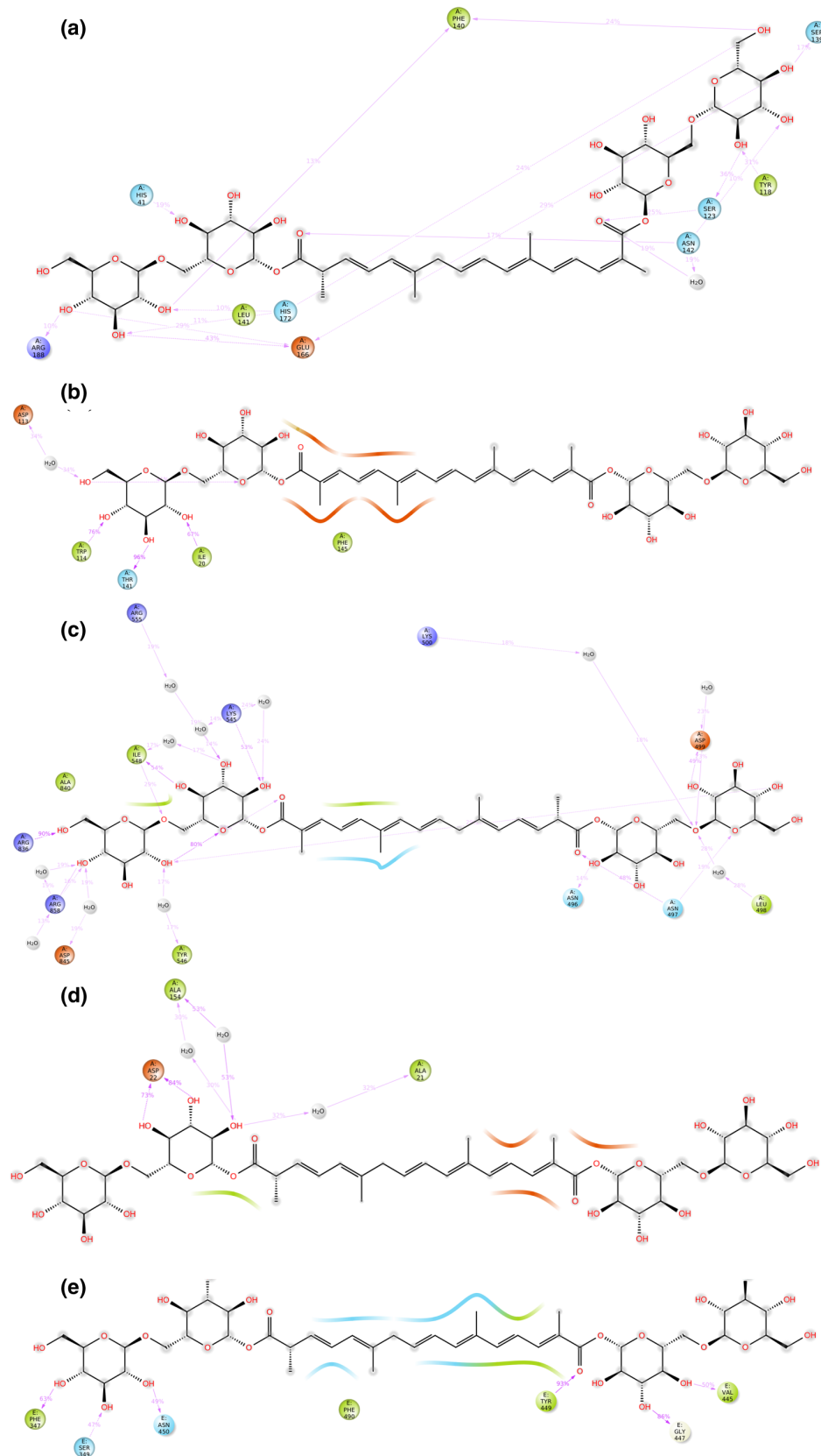
FIGURE 2 The protein–ligand contacts observed after performing 100ns MD simulation for all the macromolecular complexes of crocin with (a) M^{P^{ro}} , (b) Helicase, (c) Replication complex, (d) ADRP, and (e) B.1.351 variant of S protein. The macromolecular residues demonstrated in green color have hydrophobic interaction, whereas sky blue-colored residues have polar interactions with the complexed ligand molecule. The orange-colored residues are negatively charged, whereas the dark blue residues are positively charged
