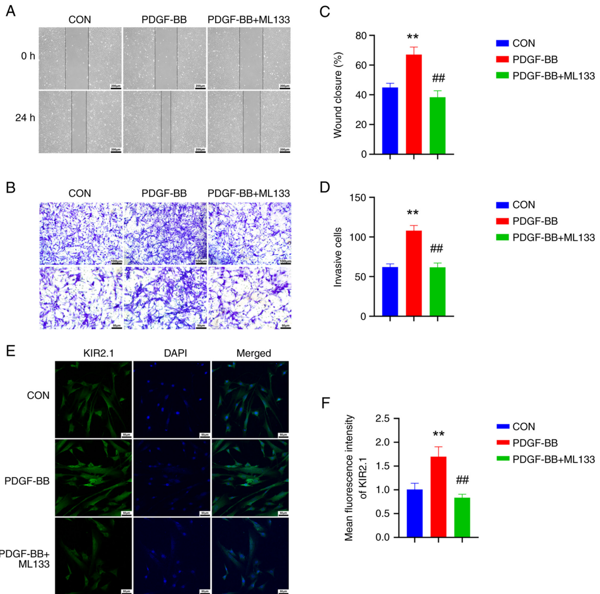
Figure 3. ML133 reverses the proliferation and migration of human pulmonary artery smooth muscle cells induced by PDGF-BB. (A) Cell scratch images; scale bar, 200 \mu\text{m} . (B) Crystal violet staining of the Transwell assay; scale bars, 100 \mu\text{m} (top panel) and 50 \mu\text{m} (bottom panel). (C) Quantitative analysis of the cell scratch healing rate. (D) Quantitative analysis of cell invasion. (E) Immunofluorescence staining for KIR2.1; scale bar, 50 \mu\text{m} . (F) Analysis of the relative expression of the KIR2.1 protein detected using immunofluorescence staining. ** P < 0.01 , PDGF-BB vs. CON; ## P < 0.01 , PDGF-BB + ML133 vs. PDGF-BB (n=6, data were analyzed using one-way ANOVA). PDGF-BB, platelet-derived growth factor-BB; KIR2.1, inwardly rectifying \text{K}^+ channel 2.1; CON, control.
