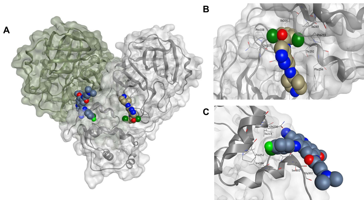
Figure 7 (A) The MPR o enzyme in the dimer form with co-crystallized ligands, (B) AT-7519 (PDB:7AGA 32 ) and (C) Pelitinib (PDB:7AXM 32 ) at the dimer interface indicates opportunities for allosteric modulation. For clarity, superimposition on the dimer form of MPR o (PDB:7CAM 79 ) was performed to demonstrate binding onto the dimerization site.
