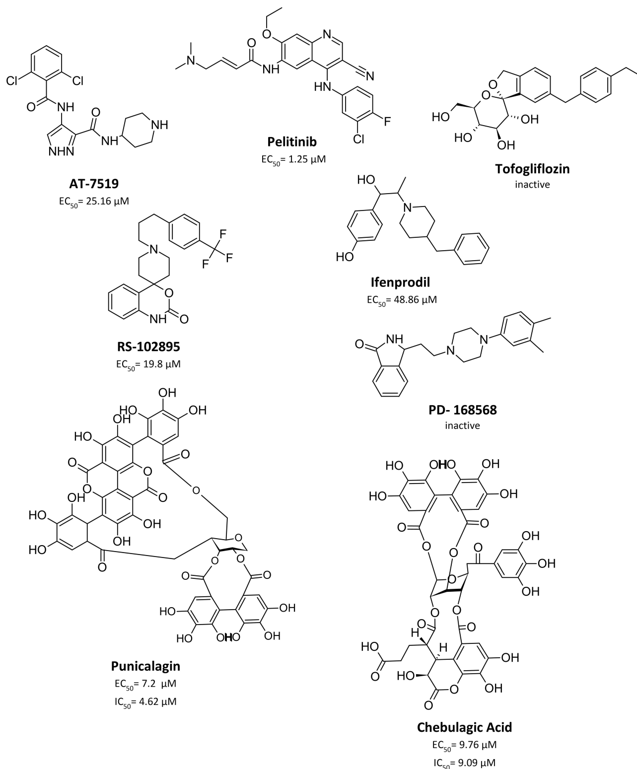
Figure 6 Chemical structure of experimentally evaluated allosteric M PPo inhibitor.
