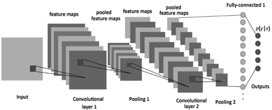
Fig. 6 Generic architecture of Convolutional neural networks [2]
