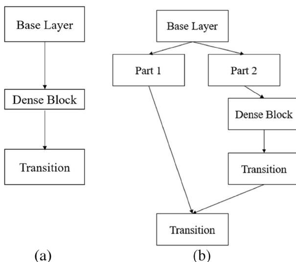
Fig. 22 CSPNet vs DenseNet architecture utilized in YOLO-v4 [73]. a CSPNet b DenseNet
