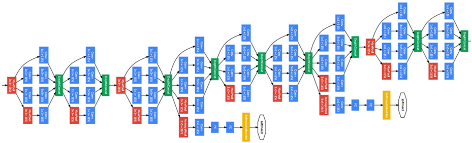
Fig. 11 GoogLeNet architecture [67]
