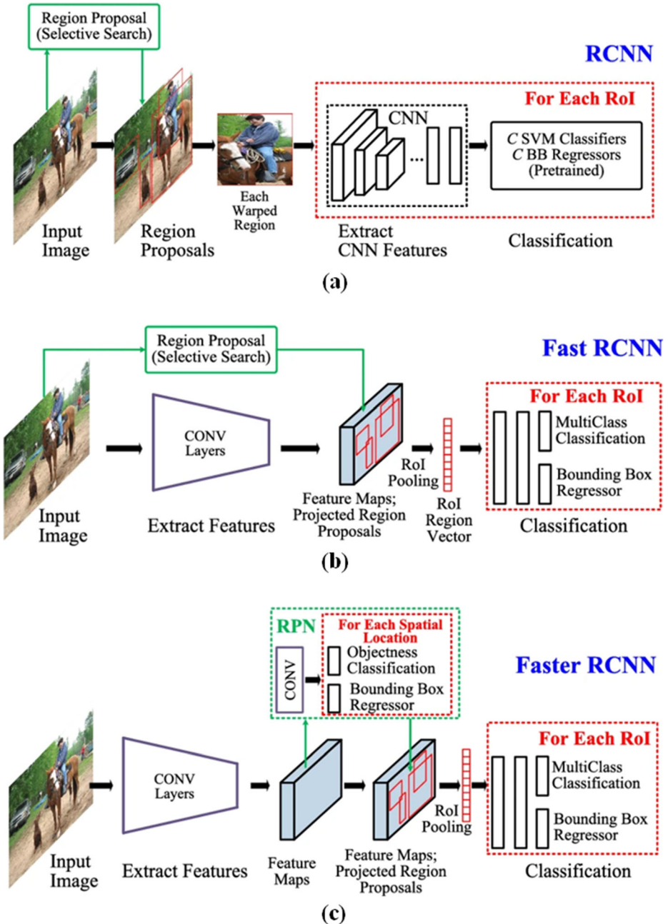
Fig. 5 Two stage object detectors (a) RCNN (b) Fast-RCNN (c) Faster-RCNN [44]
