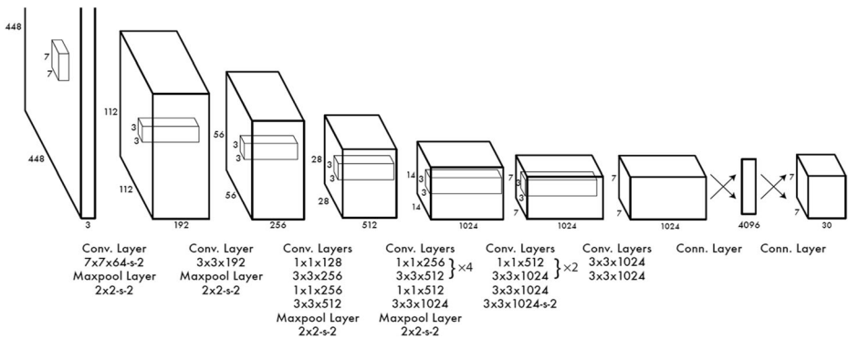
Fig. 18 YOLO architecture for object detection and localization [56]
