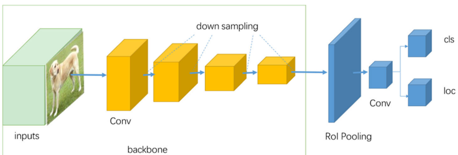
Fig. 2 Generic architecture of single stage object detectors [29]
