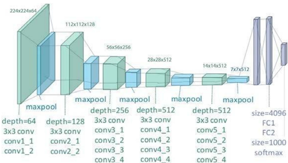
Fig. 8 VGG architecture [50]
