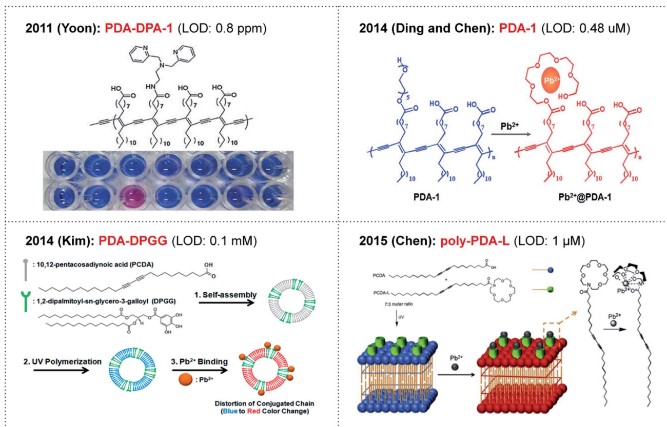
Fig. 1 Representative PDA-based colorimetric sensors for \text{Pb}^{2+} detection.
