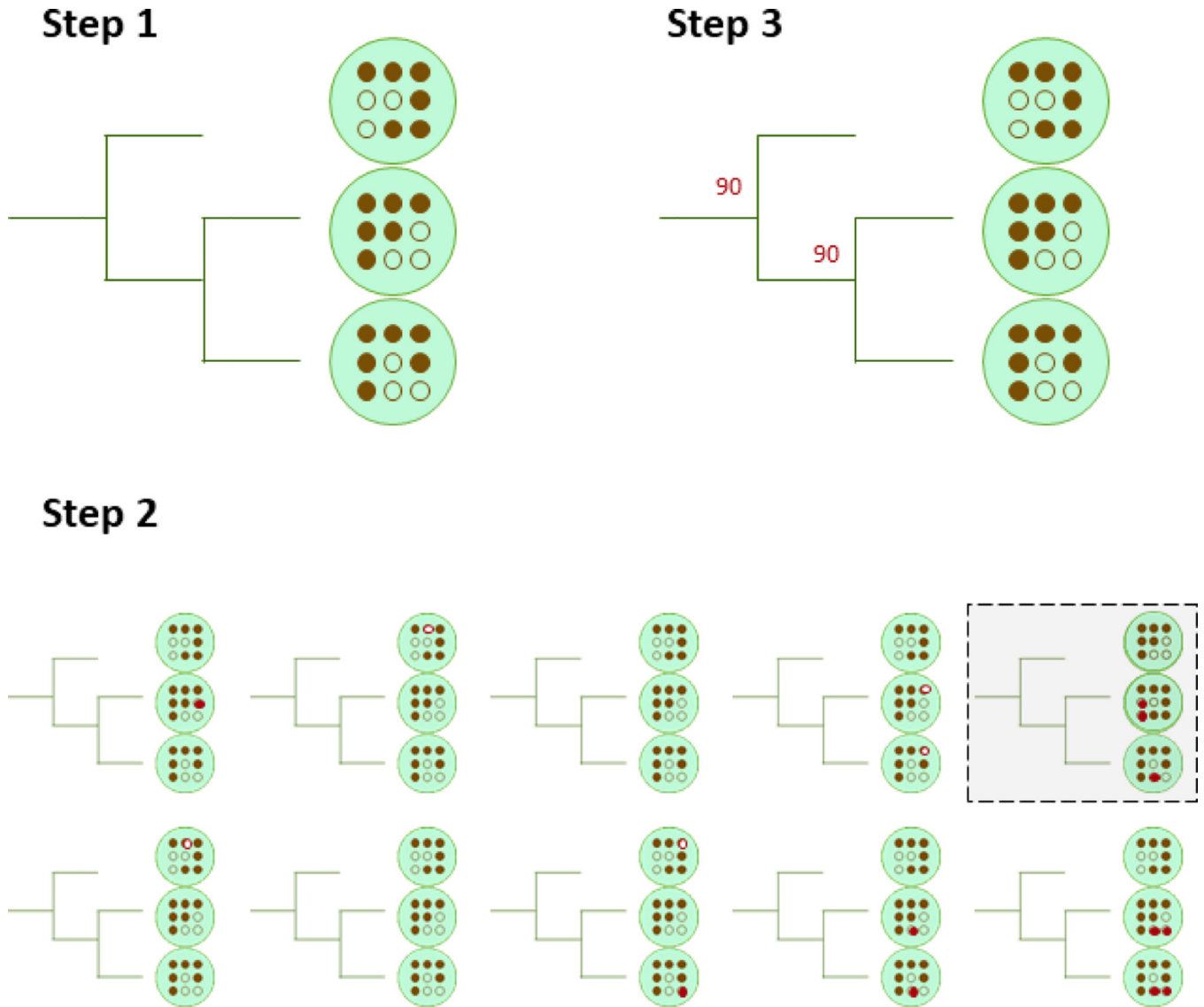
Figure 2: The Mashtree bootstrap workflow. Step 1) Generate a tree with the normal workflow as in Figure 1. This is the main tree. Step 2) Run the normal workflow once per replicate but with a different random seed. In this example, the top right replicate differs from the main tree. All ten of these trees are the bootstrap tree replicates. Step 3) For each parent node in the main tree, quantify how many bootstrap tree replicates have the same node with the same children. Record that percentage next to each parent node. This percentage quantifies how confident the Mashtree cluster is, controlling for the random seed in the Mash program.
