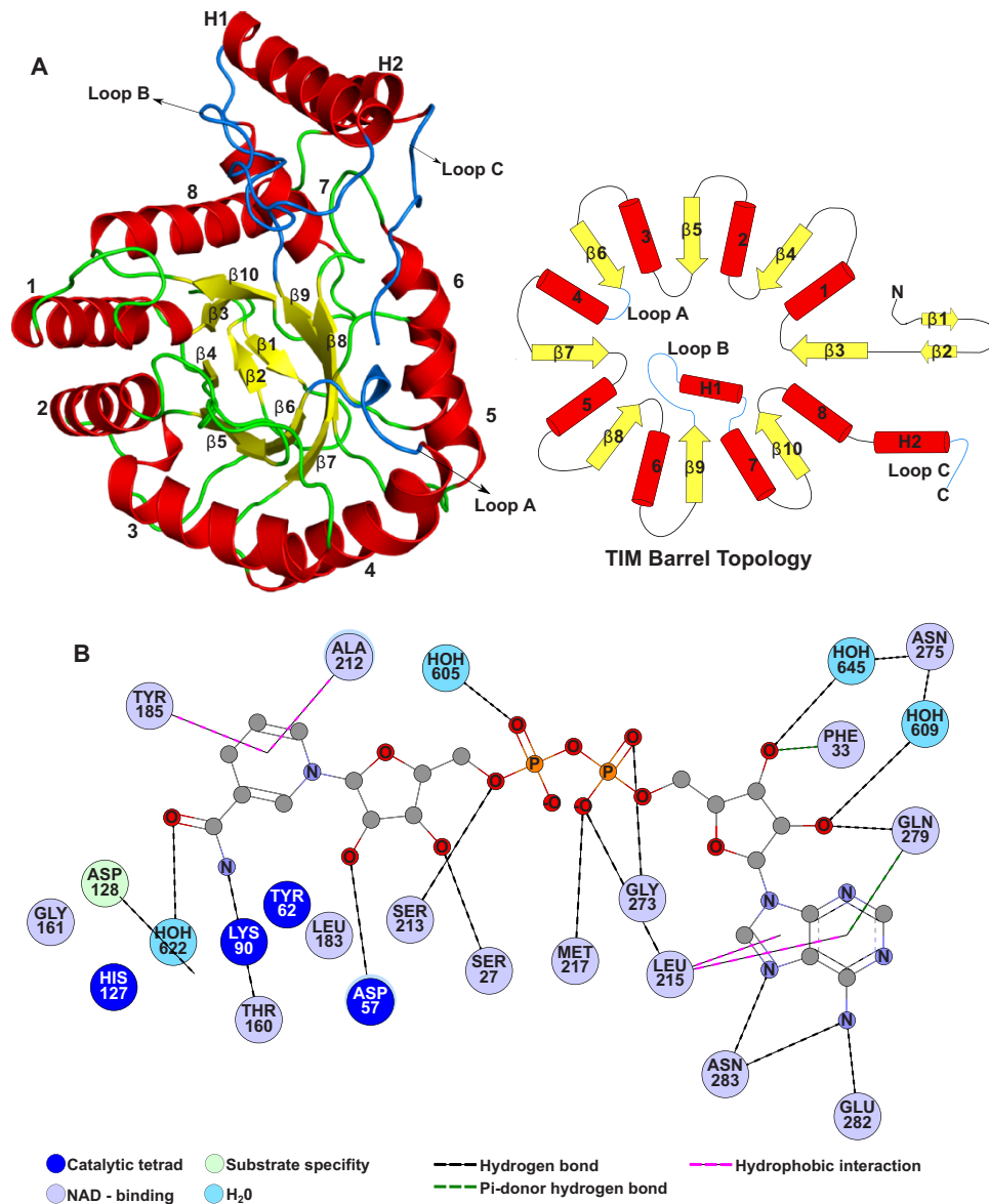
Fig. 2 SoGDH fold and NAD + -binding interactions. (A) Cartoon representation (left) and topology diagram (right) for the structure of SoGDH, which shows a (β/α) 8 -barrel (TIM-barrel) fold, characteristic of the AKR superfamily. This fold has eight β-strands interspersed by eight α-helices. At the bottom of the barrel, at the N-terminus of the polypeptide chain, there is a β-hairpin composed of strands β1 and β2. In addition, SoGDH presents two helices (H1 and H2) external to the barrel, which together with the loops loop-A, loop-B and loop-C are important for the classification of the members of AKRs. (B) The network of interactions with the NAD + cofactor. Figures were generated with PyMol v2.05 (Schrödinger, LLC, San Diego, CA, USA) and Discovery Studio Visualizer V21.1.0 (BIOVIA, Dassault Systèmes, Waltham, MA, USA).
