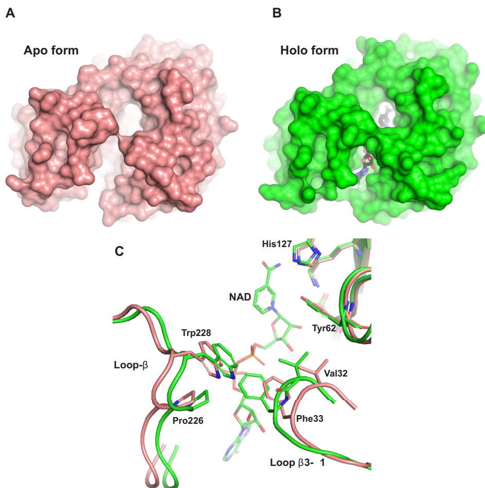
Fig. 7 The open and close states of SoGDH. (A) The apo form of SoGDH shows the open state, with little contact between loop-B and loop- \beta 3- \alpha 1. (B) The holo form of SoGDH-NAD + shows the closed state, forming a tunnel generated by the contact made between loop-B and loop- \beta 3- \alpha 1 (NAD + is shown within the tunnel at the bottom). (C) A superposition between SoGDH apo and holo forms shows a close-up of the loop-B and loop- \beta 3- \alpha 1 regions. NAD + -binding results in hydrophobic contacts between Val32, Phe33, Pro226 and Trp228, as well as hydrogen bonding between the indole nitrogen of Trp228 and the Val32 main chain.
