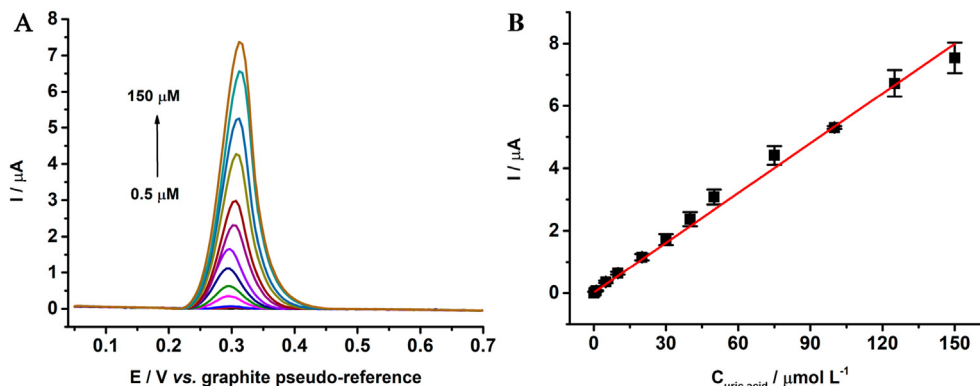
Fig. 6. Differential pulse voltammograms for increasing concentrations of UA ( 0.5, 1.0, 5.0, 10.0, 20.0, 30.0, 40.0, 50.0, 75.0, 100.0, 125.0 and 150.0 \mu\text{mol L}^{-1} ) in 0.1 \text{ mol L}^{-1} BR buffer (pH 2.0). DPV parameters: 80 mV (modulation amplitude); 30 ms (modulation time); 5 mV (step potential).
