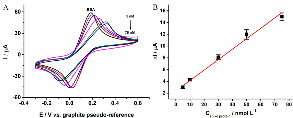
Fig. 8. Cyclic voltammograms recorded in presence of 1.0 \text{ mmol L}^{-1} FcMeOH in 0.1 \text{ mol L}^{-1} KCl using the fabricated immunosensor for increasing concentrations of antigen (5.0, 10.0, 30.0, 50.0 and 75.0 \text{ nmol L}^{-1} ); Scan rate: 100 \text{ mV s}^{-1} .
