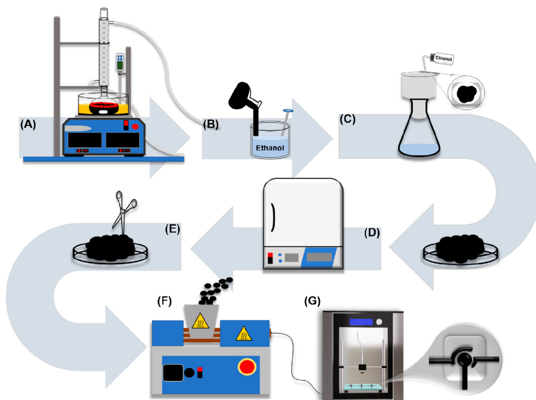
Fig. 1. Representative scheme for the production of the improved Gpt-PLA conductive filaments. (A) incorporation of graphite powder on PLA and a reflux system under constant stirring and heating; (B) recrystallization of the composite (Gpt-PLA) in ethanol; (C) filtration of the composite constantly washing with ethanol; (D) drying step on the oven at 50 °C; (E) cut into small parts; (F) composite extrusion step and (G) 3D printing of the electrochemical sensor.
