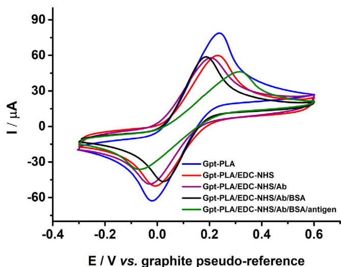
Fig. 7. Cyclic voltammetric recordings in presence of 1.0 \text{ mmol L}^{-1} FcMeOH in 0.1 \text{ mol L}^{-1} KCl after each immobilization step. Scan rate: 100 \text{ mV s}^{-1} .
