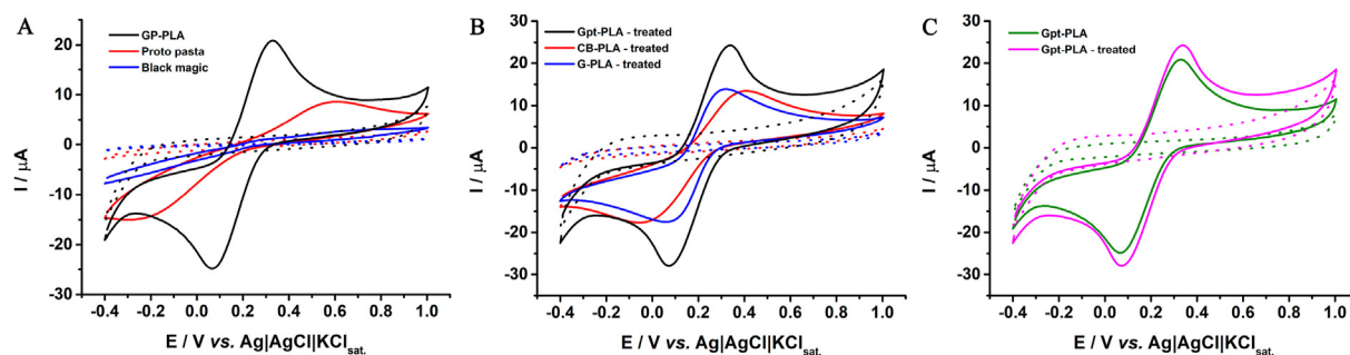
Fig. 4. Cyclic voltammograms for 1.0 \text{ mmol L}^{-1} [\text{Fe}(\text{CN})_6]^{3-/4-} in 0.1 \text{ mol L}^{-1} \text{ KCl} in A) Gpt-PLA, CB-PLA, and G-PLA after polishing in sandpaper; B) Gpt-PLA, CB-PLA, and G-PLA after electrochemical pre-treatment and; C) Gpt-PLA before and after electrochemical treatment. Scan rate: 50 \text{ mV s}^{-1} .
