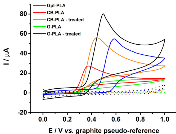
Fig. 5. Cyclic voltammograms for 1.0 \text{ mmol L}^{-1} UA in 0.1 \text{ mol L}^{-1} BR buffer (pH 2.0) on 3D printed Gpt-PLA and G-PLA and CB-PLA before and after electrochemical pre-treatment. Scan rate: 50 \text{ mV s}^{-1} .
