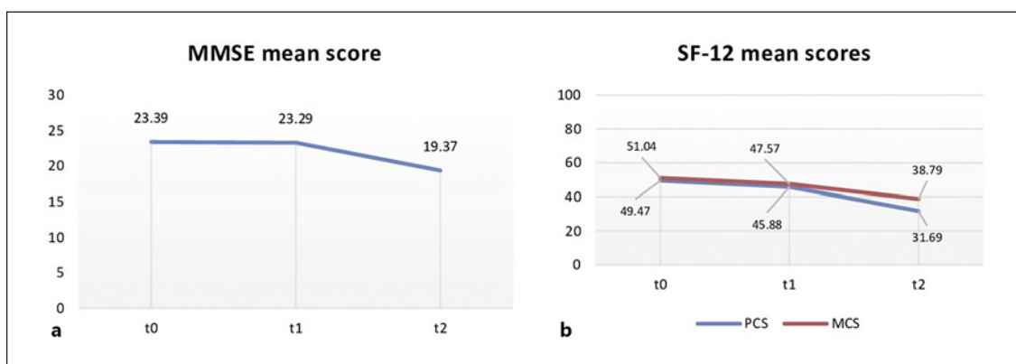
Fig. 1. Differences in cognitive performances, as expressed by the mean MMSE score (a), and in quality of life domains, as expressed by the two synthetic components of the SF-12 (b), between the three evaluation times (t0, t1, and t2). The two synthetic components were the PCS and the MCS.
