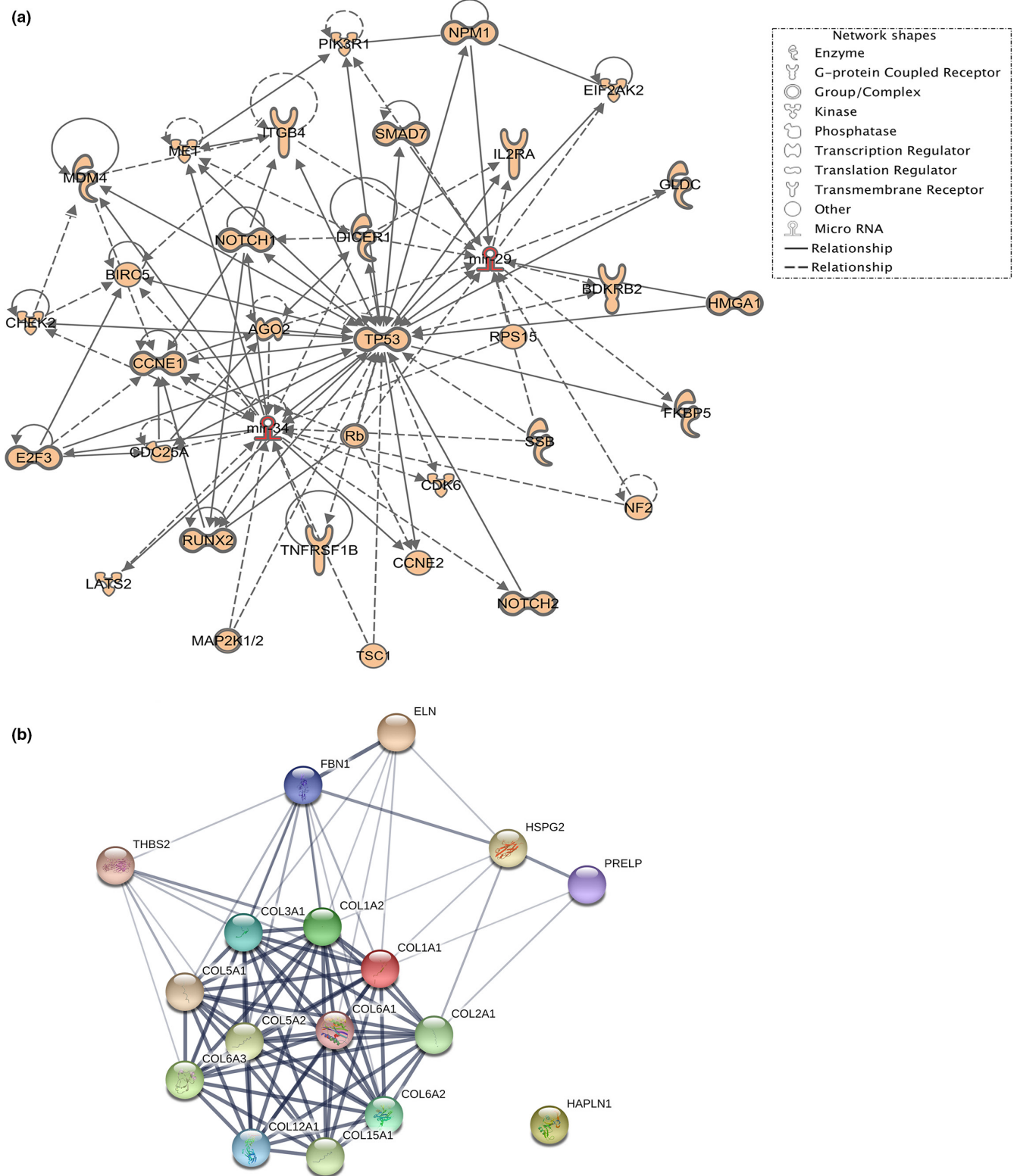
FIGURE 3 (a) Network of interactions constructed for the microRNA targets (miR-29a and miR-34a) using ingenuity pathway analysis software. (b) An interaction map of extracellular matrix target genes predicted through target scan to be upregulated by both miR-29a and miR-34a was built with STRING. One highly connected cluster was evident around collagen proteins, and a high confidence level (0.0700) was allowed for experimentally predicted gene–gene interaction.
