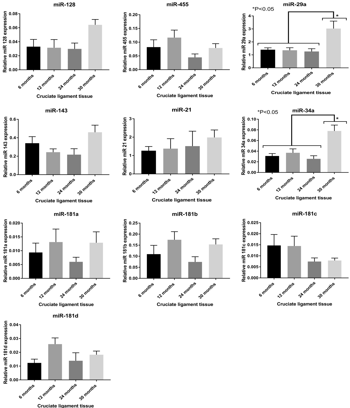
FIGURE 2 MicroRNA (miR) relative expression (to housekeeping gene Rnu6 ) at different ages in murine cruciate ligaments. Statistically significantly higher expression of miR-29a and miR-34a was found in 30-month-old mice in comparison with the 6-, 12-, and 24-month-old mice. Data are means \pm SEM.
