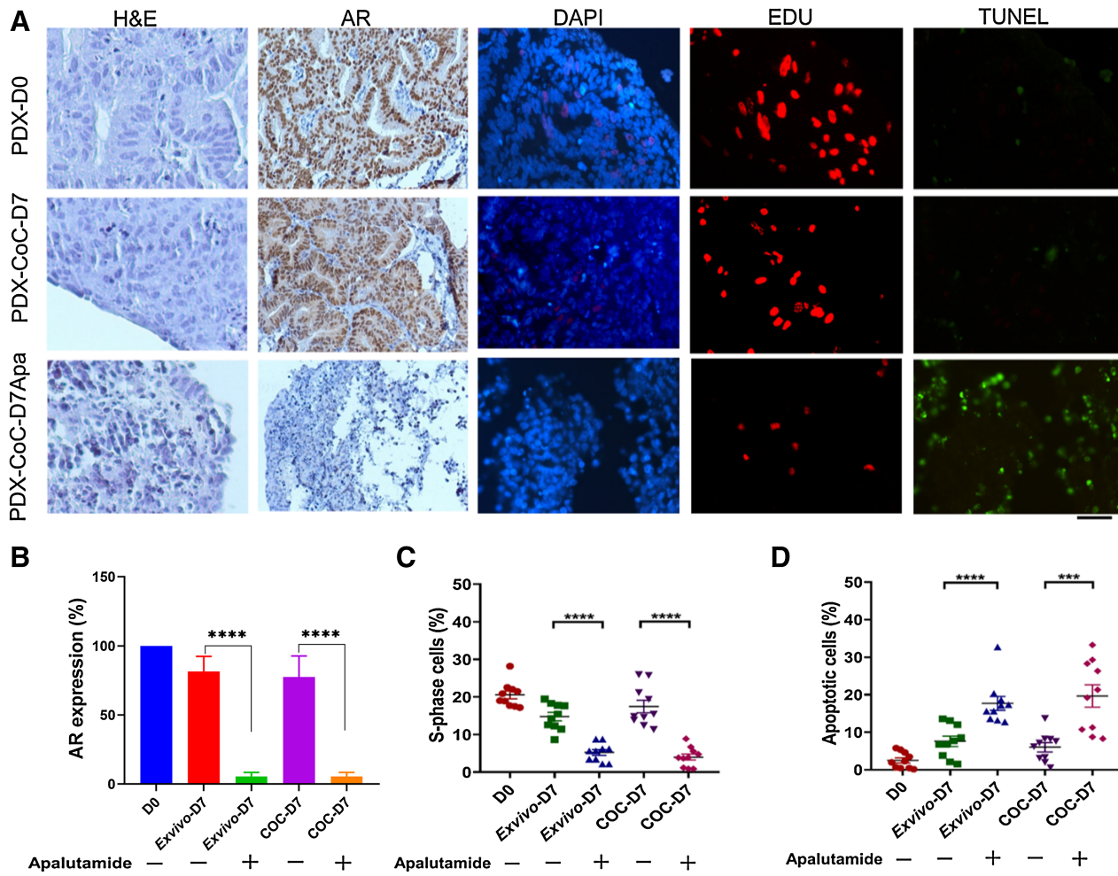
Figure 3. Response to apalutamide treatment in CoC platform. A , PC82 tumor tissue slices cultured with apalutamide for 7 days and evaluated for AR expression, cell proliferation (EdU incorporation, red nuclei), and apoptosis (TUNEL staining, green nuclei). AR staining for PC82 tissue slice sections at day 0, day 7 ex vivo culture condition, and CoC platform with and without apalutamide treatment. DAPI stains all nuclei blue. H&E, hematoxylin and eosin. Scale bar, 50 \mu m. B , Quantification of the AR expression in prostate PDX slices cultured in ex vivo and CoC platform. C and D , Apalutamide treatment showed a significant increase in TUNEL-positive cells and significant decrease in EdU-positive cells when compared with untreated tumor slices in our CoC platform. Ten fields of view were quantified per prostate PDX slice. Each point in the graph represents one image field and SEM is indicated for 10 fields. D7, day 7; D0, day 0. ***, P < 0.001 ; ****, P < 0.0001 .
