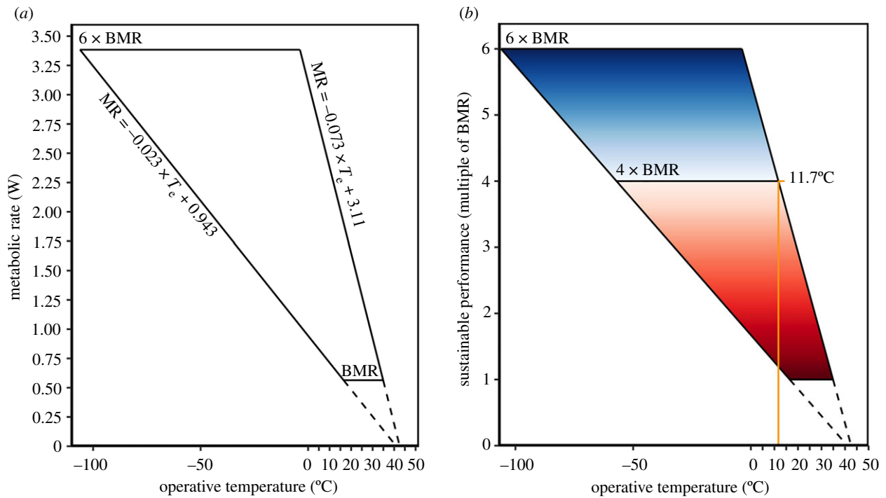
Figure 2. (a) Snow bunting ( Plectrophenax nivalis ) thermoregulatory polygon bounded by BMR (0.564 W), minimum wet thermal conductance (0.023 W/°C), maximum dry thermal conductance (0.073 W/°C) and maximal sustained metabolic rate set at 6 \times BMR. (b) Sustainable performance (expressed as a multiple of BMR) is possible for buntings under thermal balance. At operative temperatures below 11.7°C, buntings can maintain thermal balance and sustain optimal performance (i.e. performance \geq 4 \times BMR). As operative temperatures increase, buntings must reduce activity, and concomitantly metabolic rate, to maintain thermal balance, resulting in a suboptimal performance (i.e. performance less than 4 \times BMR). Optimal performance is defined as the sustained level of work required by adults to sufficiently rear nestlings. The continuous colour scheme signifies the transition into more detrimental impacts on sustainable performance at higher temperatures (i.e. dark red zone). The black dashed lines are the extrapolation of the minimum and maximum thermal conductance slopes to the average body temperature recorded during laboratory measurements. (Online version in colour.)
