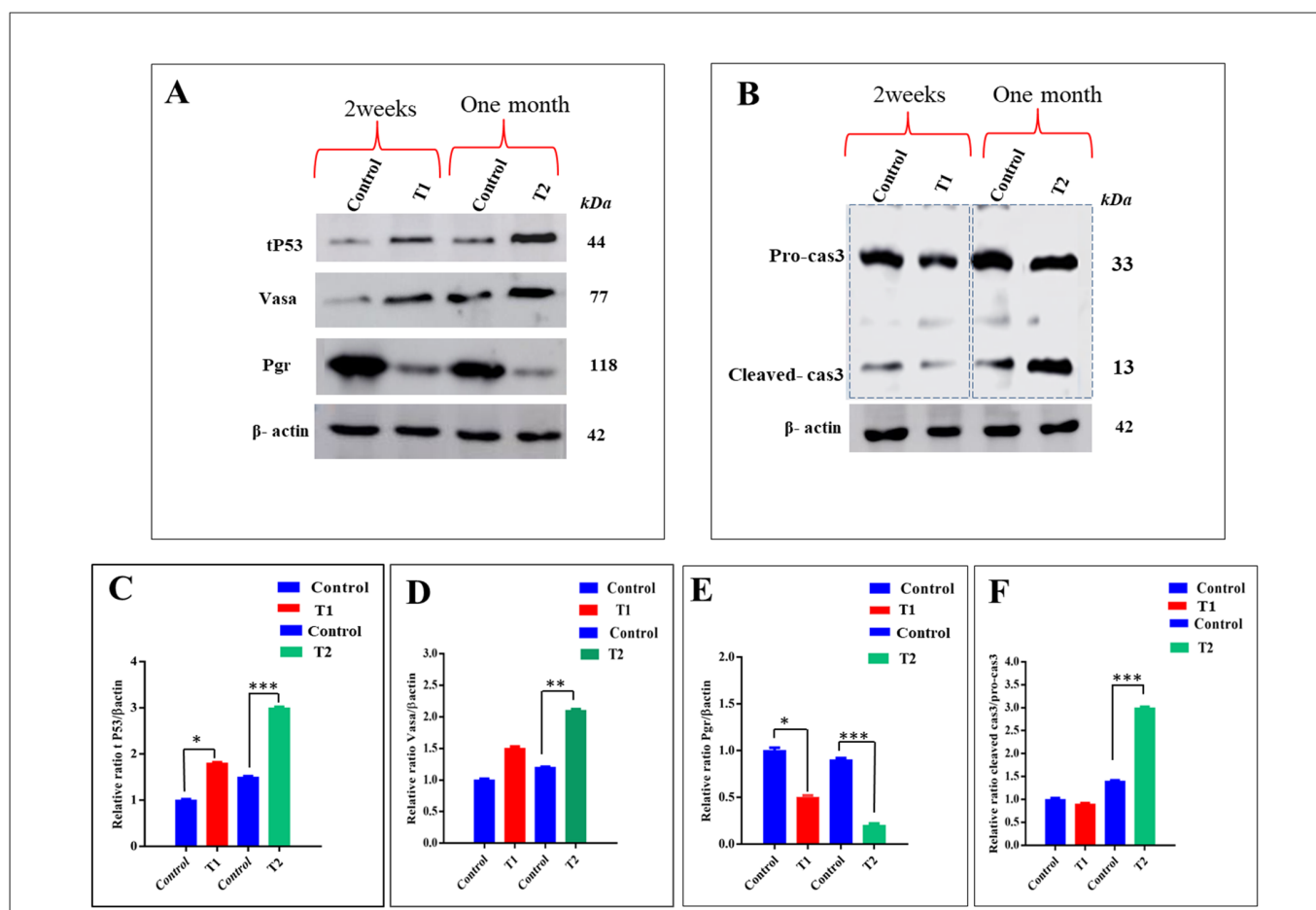
Figure 8. Effect of ZnO-NPs on necroptosis via mutated tP53 formation: (A) Western blot analysis of the tP53 protein, Vasa protein, and Pgr protein normalized to \beta -actin in control, T1, and T2 groups. (B) Western blot analysis of procaspase-3 and cleaved caspase-3 in the control, T1, and T2 groups revealed the overexpression of cleaved caspase-3 in T2 compared with the control and T1 groups. (C–F) Quantified protein expression revealed the ratio analysis of tP53/ \beta -actin, Vasa/ \beta -actin, Pgr/ \beta -actin, and cleaved-cas3/pro-cas3, respectively quantified by the Image J software. Data expressed as mean \pm SEM. * p < 0.05 , ** p < 0.01 , and *** p < 0.001 . T1 = group was exposed to 1/5th of the estimated LC 50 of ZnO-NPs in water daily for two weeks (15 days). T2 = group was exposed to 1/5th of the estimated LC 50 of ZnO-NPs in water daily for one month (30 days).
