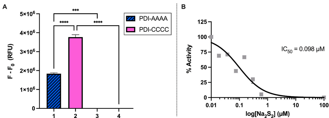
Fig. 7. A) Fluorescence intensity difference between 97 \mu\text{M} \text{Na}_2\text{S}_2 -treated (1) PDI-AAAA or (2) PDI-CCCC and untreated (3) PDI-AAAA or (4) PDI-CCCC. SSP4 (5 \mu\text{M} ) was incubated with the proteins (5 \mu\text{M} ) for 30 min at room temperature in the dark. Results are expressed as mean \pm SEM ( n = 3 ). Statistical analyses were performed using one-way ANOVA. **** P < 0.0001 , *** P = 0.0001 . B) Inhibition of PDI reductase activity by \text{Na}_2\text{S}_2 . PDI (0.2 \mu\text{M} ) was incubated with the indicated concentration of \text{Na}_2\text{S}_2 and assayed for reductase activity using a di-eosin-GSSG assay.
