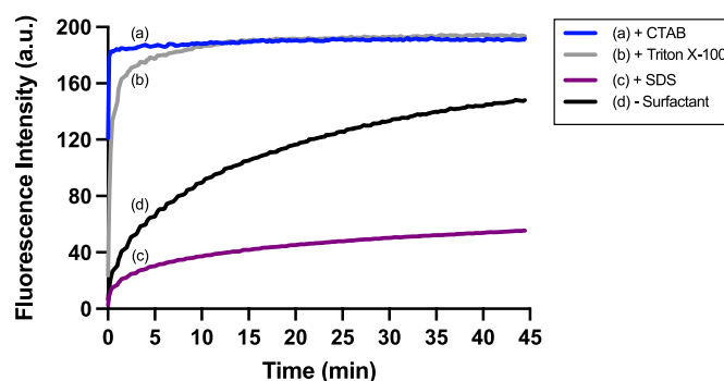
Fig. 1. Time-dependent response of SSP4 (5 \mu\text{M} ) to \text{Na}_2\text{S}_2 (25 \mu\text{M} ) in 50 mM PBS buffer (pH 7.4) and (a) CTAB, (b) Triton X-100, (c) SDS (25 \mu\text{M} ), or (d) no surfactant at room temperature. Emission: 514 nm, excitation: 482 nm.
