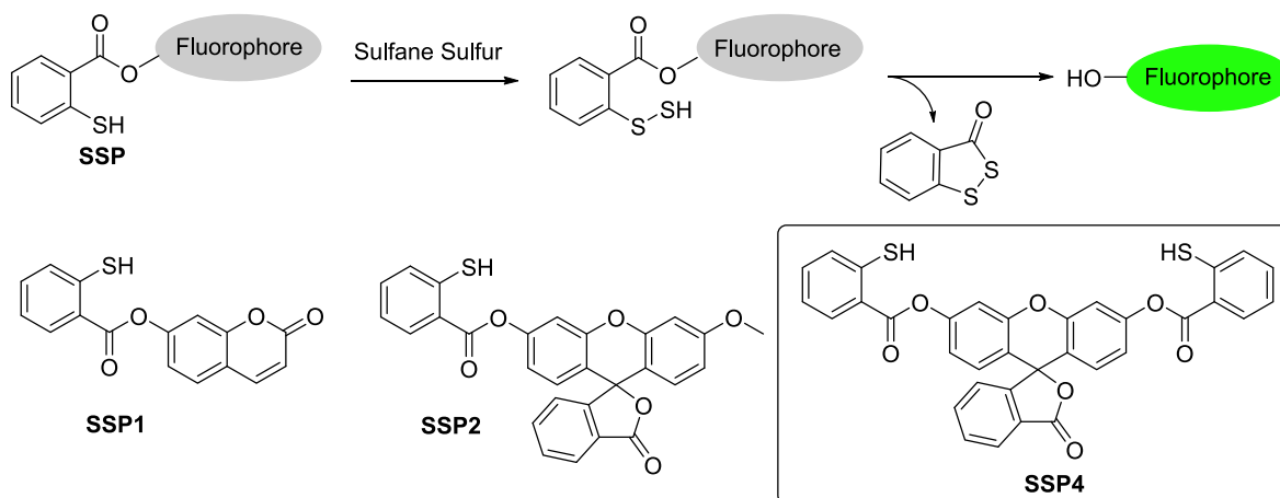
Scheme 1. The structures and reaction of SSP fluorescent probes.
