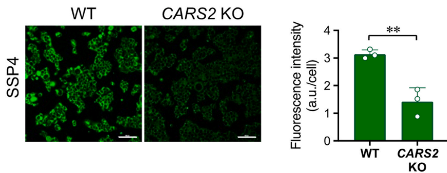
Fig. 8. Representative cell images with SSP4. (I) Brightfield (A, D), fluorescence (B, E), and overlaid images (C, F) of \text{H}_2\text{S}_2 in HeLa cells. Cells were first treated with 5 \mu\text{M} of SSP4, then washed and subjected to (A–C) No \text{Na}_2\text{S}_2 added, (D–F) 50 \mu\text{M} \text{Na}_2\text{S}_2 . (II) COS-7 cells overexpressing CSE and WT and (III) CARS2 KO HEK293T were subjected to fluorescence staining. Fluorescence images (left panel) and fluorescence intensities (right panel) of SSP4 staining. Scale bars, 100 \mu\text{m} . Data are mean values \pm S.D (from three different images, each containing more than 100 cells in a representative experiment). * P < 0.05 , ** P < 0.01 ; Student's t -test.
