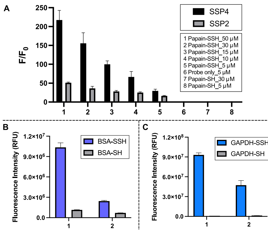
Fig. 6. (A) Fluorescence enhancement ( F/F_0 ) of 5 \mu\text{M} SSP4 or SSP2 in the presence of varied concentrations of persulfidated papain. (B)/(C) Fluorescence intensity of 5 \mu\text{M} SSP4 for the detection of various concentrations of persulfidated and reduced BSA or GAPDH at (1) 30 \mu\text{M} and (2) 5 \mu\text{M} . Results are expressed as mean \pm SEM ( n = 3 ).
