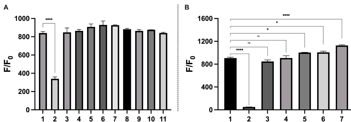
Fig. 5. Mean fluorescence enhancements of SSP4 (5 \mu\text{M} ) with 25 \mu\text{M} S 8 in the presence of (A) various analytes: (1) control; (2) 1 mM GSH; (3) 200 \mu\text{M} Hcy; (4) 30 \mu\text{M} methionine (Met); (5) 100 \mu\text{M} Cys; (6) 100 \mu\text{M} GSH; (7) 100 \mu\text{M} N -acetyl-L-cysteine (NAC); (8) 150 \mu\text{M} glycine (Gly); (9) 55 \mu\text{M} tyrosine (Tyr); (10) 40 \mu\text{M} tryptophan (Trp), (11) 100 \mu\text{M} arginine (Arg). (B) metal ions: 1) control; (2) CuSO 4 ; (3) FeCl 2 ; (4) FeCl 3 ; (5) MgCl 2 ; (6) CaCl 2 ; (7) ZnCl 2 at 20 equivalents (500 \mu\text{M} ) to the 25 \mu\text{M} S 8 . Results are expressed as mean \pm SEM ( n = 3 ). Statistical analyses were performed using one-way ANOVA. **** P < 0.0001 , * P = 0.0326 – 0.0431 , ns = not significant.
