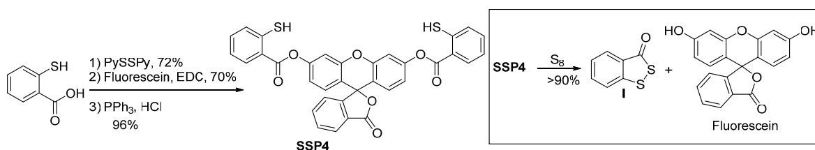
Scheme 1. The structures and reaction of SSP fluorescent probes.
