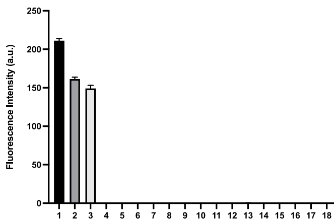
Fig. 4. Mean fluorescence response of SSP4 (5 μM) in the presence of: (1) 25 μM cysteine polysulfide (Cys-polysulfide); (2) 25 μM sodium disulfide (Na 2 S 2 ); (3) 25 μM elemental sulfur (S 8 ); (4) 1 mM L-cysteine (Cys); (5) 1 mM glutathione (GSH); (6) 1 mM homocysteine (Hcy); (7) 30 μM methionine (Met); (8) 100 μM N-acetyl-L-cysteine (NAC); (9) 100 μM oxidized glutathione (GSSG); (10) 100 μM sodium sulfate (Na 2 SO 4 ); (11) 100 μM sodium thiosulfate (Na 2 S 2 O 3 ); (12) 100 μM sodium sulfite (Na 2 SO 3 ); (13) 100 μM sodium sulfide (Na 2 S); (14) 150 μM glycine (Gly); (15) 55 μM tyrosine (Tyr); (16) 40 μM tryptophan (Trp); (17) 100 μM arginine (Arg); (18) probe only. Results are expressed as mean ± SEM ( n = 3).
