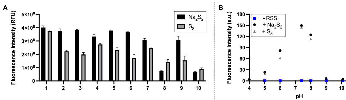
Fig. 2. Fluorescence responses of SSP4 (5 μM) toward Na 2 S 2 or S 8 (25 μM) in (A) different buffers: (1) 50 mM PBS, pH 7.4; (2) 10 mM PBS, pH 7.4; (3) 50 mM Tris buffer, pH 7.4; (4) 50 mM sodium phosphate buffer, pH 7.4; (5) 50 mM potassium phosphate buffer, pH 7.0; (6) 50 mM HEPES (7) Fluorobrite DMEM; (8) Fluorobrite DMEM + 10% FBS; (9) DMEM; (10) DMEM + 10% FBS. (B) different pHs in 50 mM PBS (pH 7.4). CTAB (25 μM) was added to all reactions, and reactions were carried out for 20 min at room temperature. Results are expressed as mean ± SEM ( n = 3).
