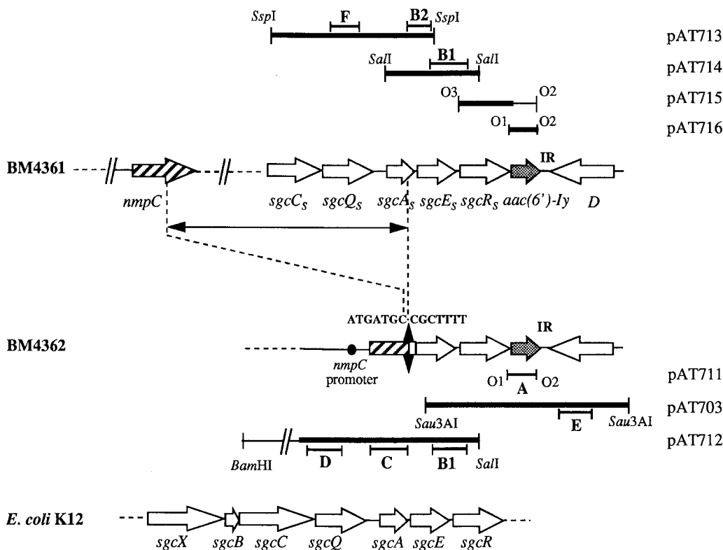
FIG. 1. Schematic representation of the environments of aac(6') -Iy in BM4361 and BM4362 and of the 97.6-min chromosomal region of E. coli K12. Arrows indicate the direction of transcription. The ORFs upstream from aac(6') -Iy in BM4361 (open arrows) had ca. 75% identity with the 97.6-min chromosomal region of E. coli K12. The nucleotides adjacent to the deletion are indicated. The inserts of recombinant plasmids are represented by lines between vertical lines, and the sequenced portions are indicated by thick lines. The oligodeoxynucleotides used for PCR amplification are indicated (O1 from 3034 to 3053, O2 from 3451 to 3470, and O3 from 2177 to 2196; the numbering is in accordance with that for the sequence with GenBank accession no. AF144881). Probes B1 and B2 used for screening recombinant plasmids and probes A to F used for Southern and Northern analyses are indicated. The ca. 60-kb deletion is indicated by a double-headed arrow.
