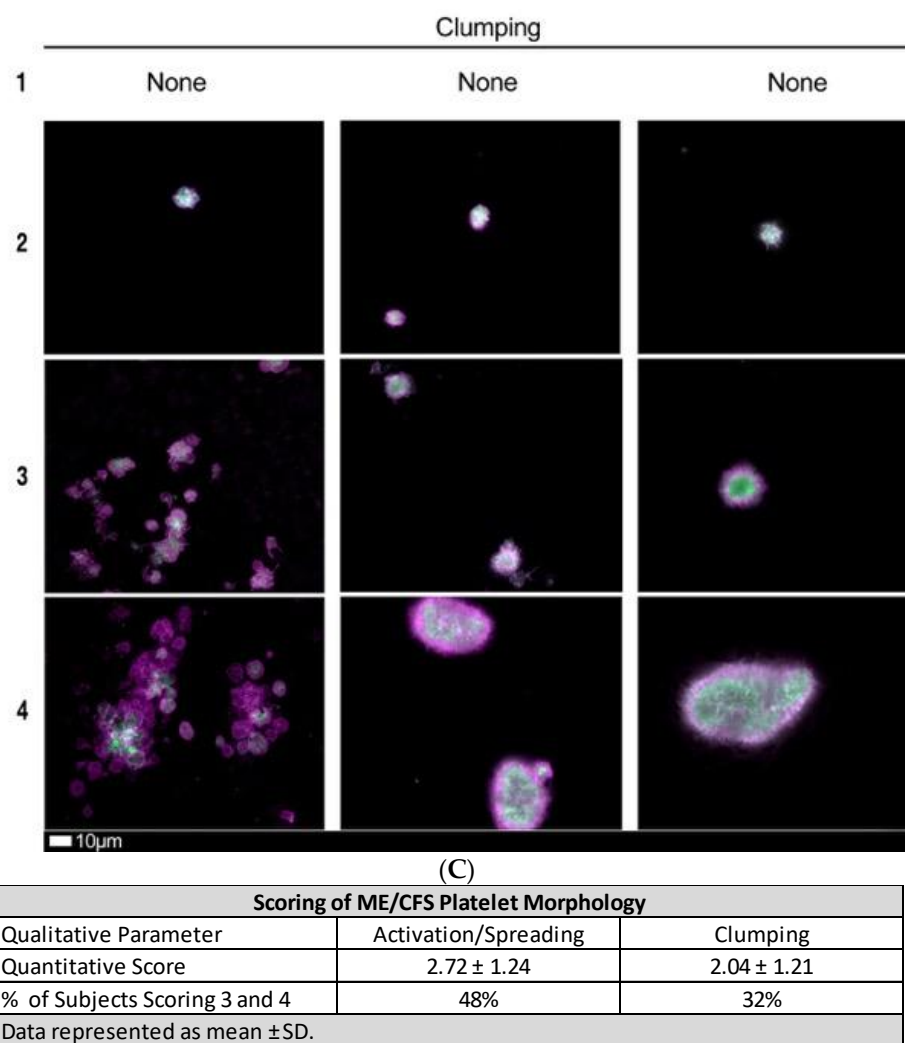
Figure 3. (A) Representative fluorescent micrographs of hematocrit samples from ME/CFS individuals stained with PAC-1 (green fluorescence) and CD62P-PE (purple fluorescence); white areas represent overlap of the two markers. Images were taken at 63\times magnification. (B) Fluorescence micrograph examples depicting the scoring system used to measure platelet activation determined by spreading, that was previously developed to score platelet activation in Long COVID/PASC patients. This scoring system functions to assign a quantitative score to qualitative data. In Stage 1 (activation with pseudopodia), platelets are minimally activated and are seen as small and round with few pseudopodia (representative of healthy/control platelets). Severe platelet activation, characterized by large, egg-shaped morphology and aggregations, is registered as Stage 4 [47] and is indicative of hyperactivated platelets. All images within a row reflect the same score. (C) Fluorescence microscopy examples of the scoring system used to assess platelet clumping. This scoring system was developed to assign a quantitative score to qualitative data. Clumping is absent in Stage 1 (representative of control samples). Conversely, severe platelet clumping is registered as Stage 4 [47]. All images within a row reflect the same score. (D) Mean quantitative scores of platelet spreading and clumping parameters in the ME/CFS group. Platelets were scored according to the scoring system depicted in Figure 3B,C.
