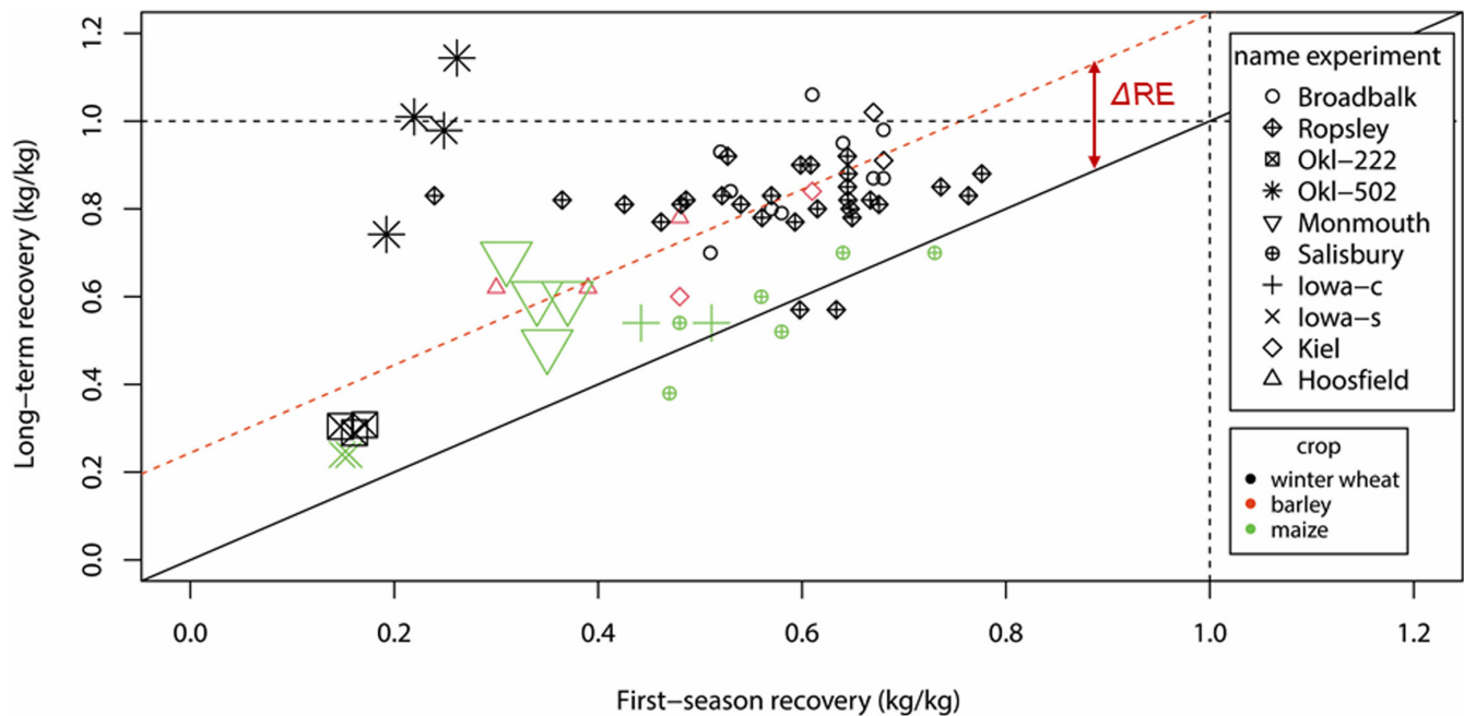
FIGURE 4 First season recovery and long-term recovery for winter wheat, spring barley and maize ( N = 66 ). The diagonal solid black line indicates RE^{LT} = RE^{1st} ; the difference between that black line and the red diagonal dashed line indicates the estimated average \Delta RE . Point-size indicates the weight based on sample size. Note that data from the LTE Bad Lauchstädt is excluded from this graph because separate values of long and first season recovery could not be calculated and \Delta RE was assessed differently (see Table S1; see Equation S2)
