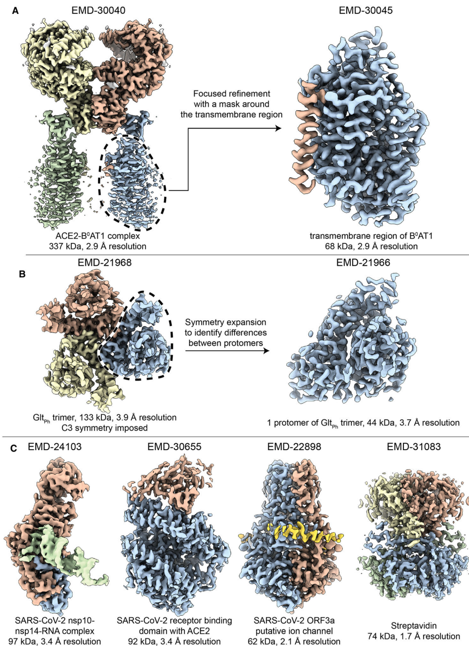
Figure 1. Some examples of recent structures that have been determined by cryo-EM.
