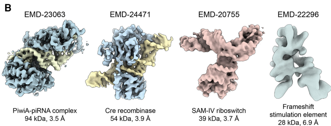
Figure 2. Illustration of the rapid growth in the ability of single-particle cryo-EM to produce high-resolution structures of small macromolecules.
