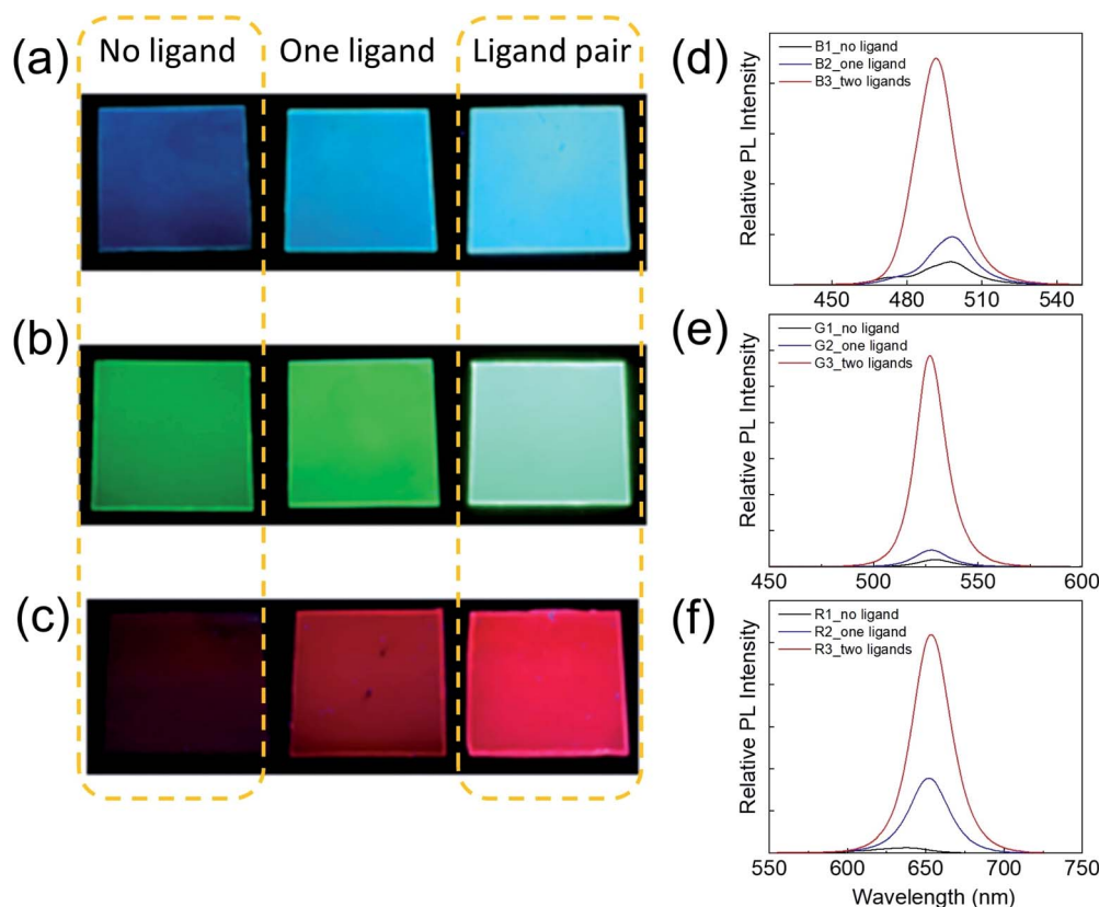
Fig. 4 (a–c) Photographs of the luminescent (a) blue (CsPbClBr 2 -PS), (b) green (CsPbBr 3 -PS) and (c) red (CsPbBrI 2 -PS) composites prepared with no ligand (left), one ligand (middle) or two ligands (right), under UV excitation. All photos are taken with identical camera exposure settings. (d–f) Comparison of PL emission spectra and relative PL intensities of (d) blue (CsPbClBr 2 -PS), (e) green (CsPbBr 3 -PS) and (f) red (CsPbBrI 2 -PS) composites prepared with no ligand (black line), one ligand (blue line) or two ligands (red line).
