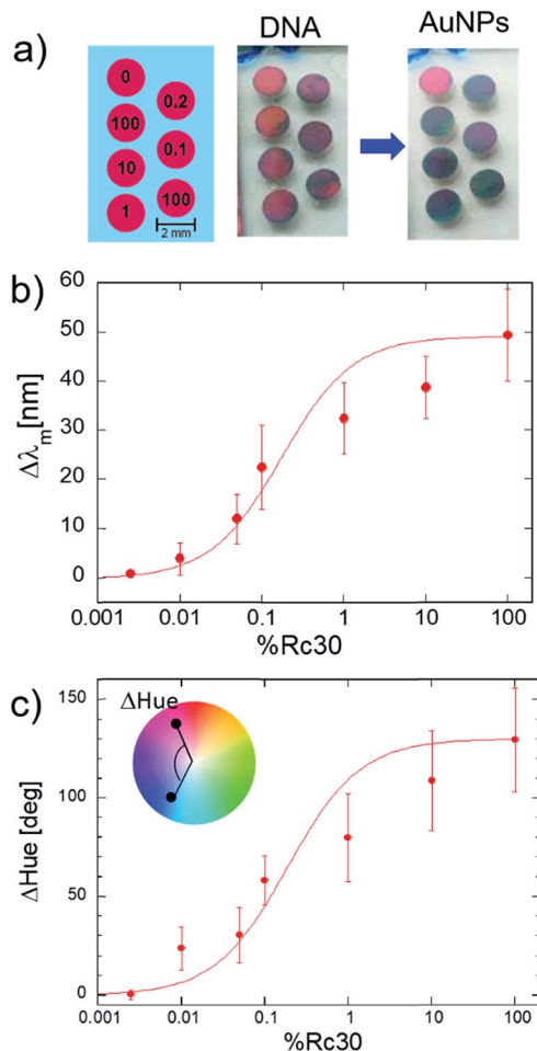
Fig. 6 (a) (Left) Sketch of the sensing spots and photographs of the sensing spots taken before (middle) and after immobilization of DNA-AuNPs (right). The quantitative plot of (b) shift amount of the resonance wavelength \Delta\lambda_m and (c) shift in the hue angle \Delta\text{hue} against the relative surface coverage of Rc30, %Rc30.
