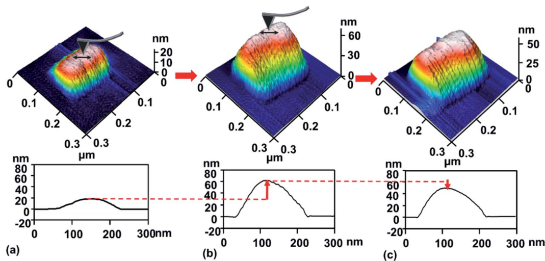
Fig. 3 Scratching tests on the hillock-like structure surface. (a) A hillock-like structure with a height of \sim 20 nm on the supported graphene surface; (b) and (c), respectively, show that after the scratching test, the height of the hillock-like structure increased from \sim 20 nm to \sim 60 nm, and then decreased from \sim 60 nm to \sim 45 nm.
