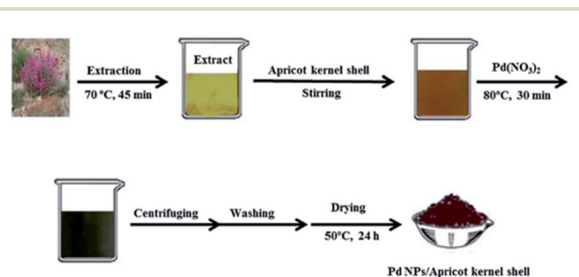
Fig. 6 Synthesis procedure of Pd NPs/Apricot kernel shell. Reprinted with permission from Elsevier. 108
