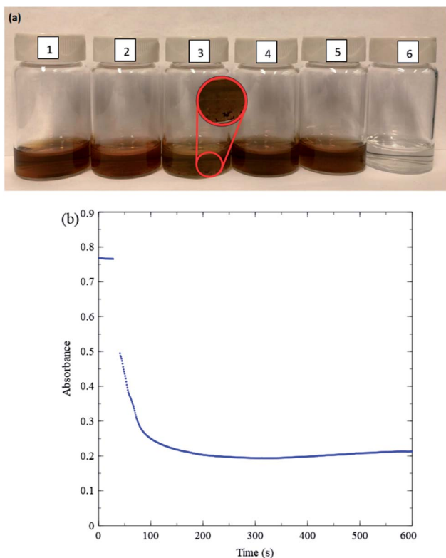
Fig. 3 (a) Photographs of various nanosheet solutions in DI-water 15 min. after preparation (1) \text{MnO}_2 ; (2) \text{MnO}_2 and HCl; (3) \text{MnO}_2 and NaCl; (4) \text{MnO}_2 , MES buffer and glucose; (5) \text{MnO}_2 , MES buffer, and gluconic acid; (6) \text{MnO}_2 , MES buffer, gluconic acid and \text{H}_2\text{O}_2 . (b) Absorbance of the nanosheets in DI-water at 384 nm vs. time upon injecting \text{H}_2\text{O}_2 . Near the \sim 30 s mark, about 15 s of data have been omitted due to absorbance fluctuations caused by opening the spectrometer lid, injecting \text{H}_2\text{O}_2 and stirring. Initial reaction rate approx. 0.022 \text{ s}^{-1} .
