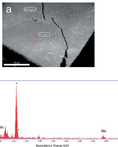
Fig. 2 (a) ESEM image of a thick \text{MnO}_2 film. (b) Energy dispersive spectrum obtained at Spot 1 shown in Fig. 2a (a spectrum obtained at Spot 2 is shown in Fig. S3†).
