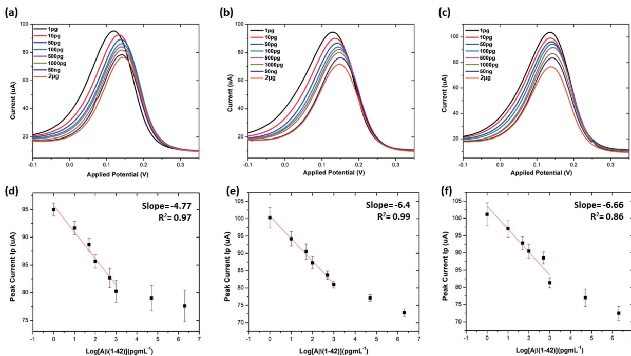
Fig. 6 Differential pulse voltammetry (DPV) results at 20 \text{ }\mu\text{g mL}^{-1} , 40 \text{ }\mu\text{g mL}^{-1} and 60 \text{ }\mu\text{g mL}^{-1} concentration of A\beta antibodies: (a–c) DPV plots of 20 \text{ }\mu\text{g mL}^{-1} , 40 \text{ }\mu\text{g mL}^{-1} and 60 \text{ }\mu\text{g mL}^{-1} antibodies at each stage of sensing; (d–f) corresponding calibration curves of I_p as against log A\beta(1-42) concentrations. All data points are mean values of three independent electrodes. The error bars (calculated as the standard deviation) provide a measure of repeatability of the system ( n = 3 ).
