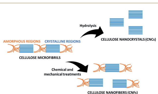
Fig. 3 Production of CNCs and CNFs from cellulose.
